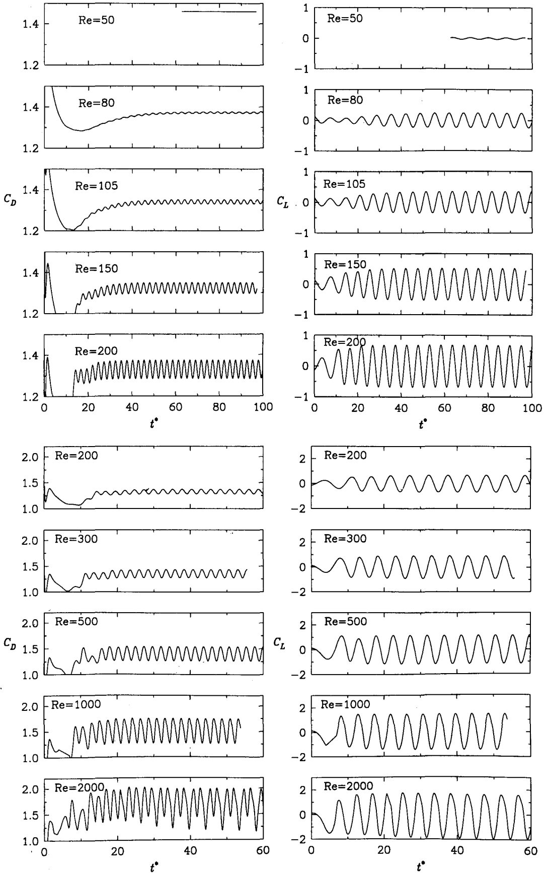
Figure 4.27: Time history of the drag coefficient (left) and the lift coefficient (right) for vortex shedding from a circular cylinder as a function of Reynolds numbers (grid D1-143x98, SMART scheme).
