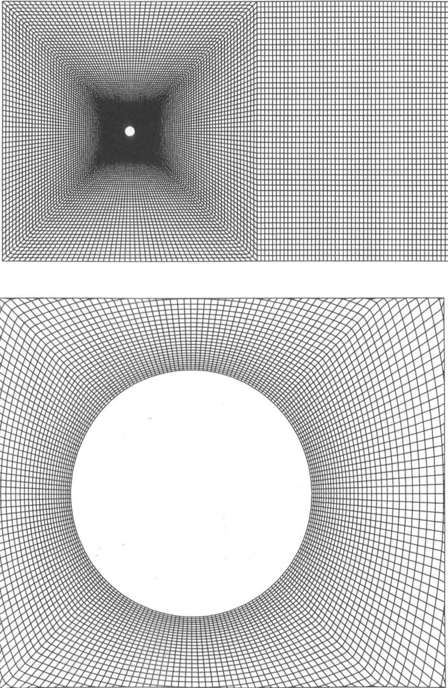
Figure 5.23: Numerical grid G1 used for the flow past a circular cylinder at Re = 1.4 \times 10^5 .
