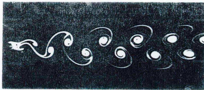
Figure 4.12: Streaklines for a circular cylinder at Re = 105 : (a) computed at t^* = 204.9 (where the lift coefficient is at maximum); (b) photograph from experiments by S. Taneda, van Dyke (1982).
