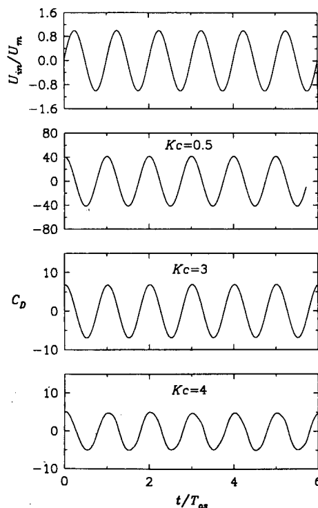
Figure 4.34: Circular cylinder in pure oscillatory flows. Computed drag coefficients versus time at Kc = 0.5, 3, \text{ and } 4 and \beta = 196 (the top curve shows the inlet velocity variation).
