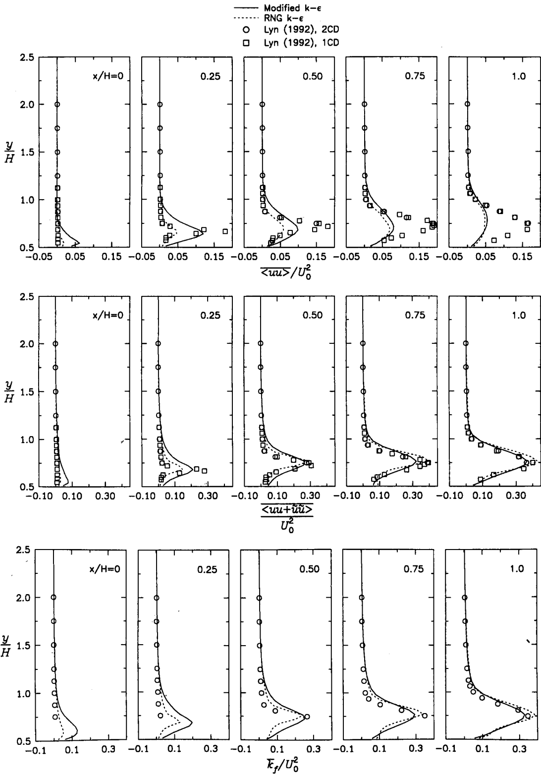
Figure 5.18: The time-averaged profiles of the Reynolds stress component \langle u^2 \rangle (top), apparent component \langle u'^2 \rangle = \langle u^2 + \tilde{u}^2 \rangle (middle) and global fluctuating kinetic energy k_f (bottom) at several lateral cross-sections along the upper side of a square cylinder.
