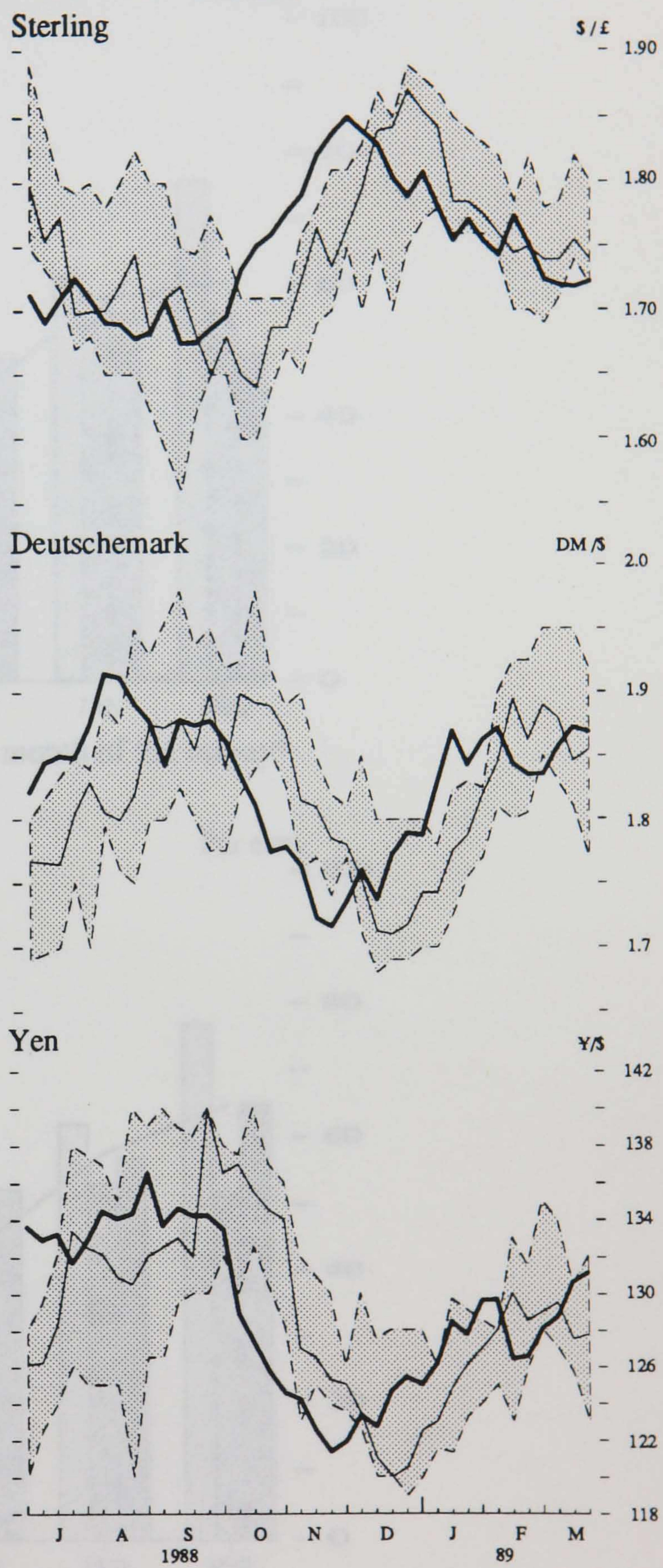
(b) Actual rate plotted at time t , forecasts plotted at time t + 4 .
