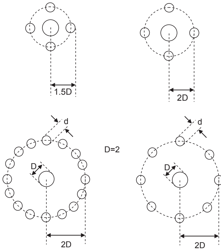
Figure 7 Details of the geometry of the novel pile groups used to investigate the influence of 1.5D and 2D centre to centre spacing between the centre pile and the mini-pile group (D – diameter of centre pile). Details of the geometry of the model of novel pile groups of 8 and 16 mini-piles.
