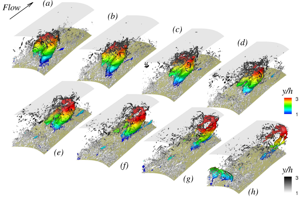
FIGURE 15. Instantaneous flow visualization around the lobe plane ( 0.0 \leq z/h \leq 4.0 ) and over the stoss side ( 7.9 \leq (x - x_s)/h \leq 20.0 ) for Case 5 (in-phase crestline alignment) at 8 instants in time between (a) tU_b/h = 164 and (h) 172. Isosurfaces of pressure fluctuations p'/\rho U_b^2 = -0.038 for (a-d) and p'/\rho U_b^2 = -0.03 for (e-h) are coloured by the distance from the bed with rainbow colormap and isosurfaces of the second invariant of the velocity tensor, Qh^2/U_b^2 = 3.78 , are coloured by the distance from the bed with grayscale colormap.
