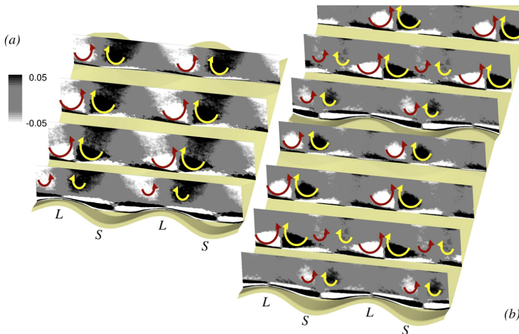
FIGURE 2. Contours of mean streamwise vorticity, \Omega_x h/U_b , for (a) Case 5 and (b) Case 11 on crossplanes at x/h = 2.0, 7.0, 12.0, 17.0, 22.0, 27.0, and 32.0 . Arrows show the mean secondary flows. “L” represents the lobe and “S” represents the saddle.
