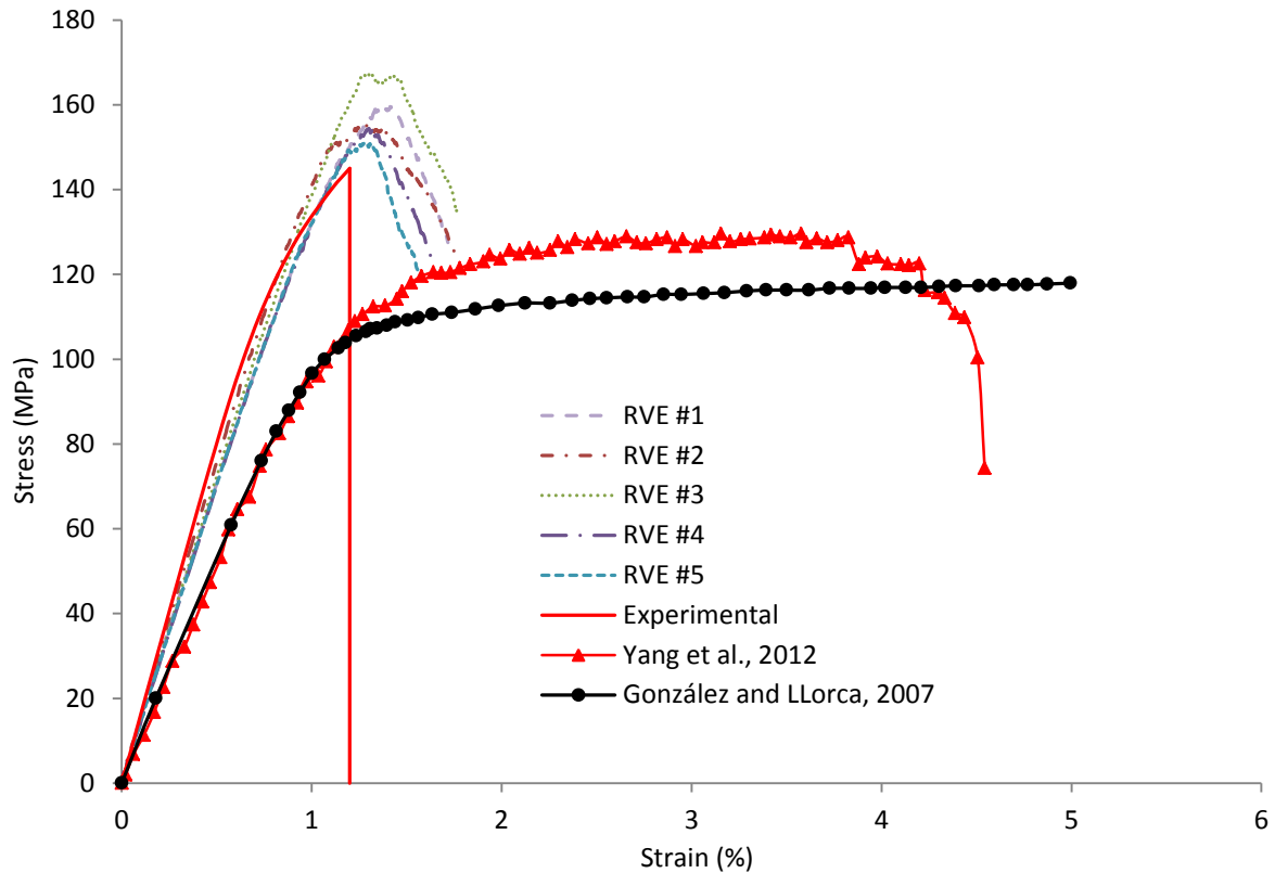
Fig.11 Stress–strain curves of five RVEs under uniaxial compression.
