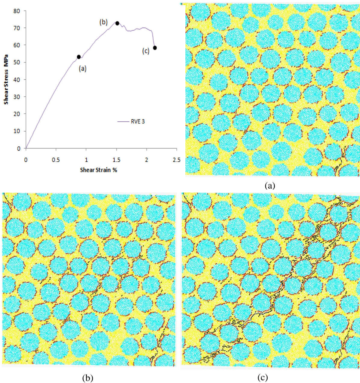
Fig.14 Damage evolution under transverse shear of RVE #3 at different strain stages: (a) 0.87%, (b) 1.51%, and (c) 2.13%. (Red dots are fibre/matrix debonding and black dots are matrix cracks)
