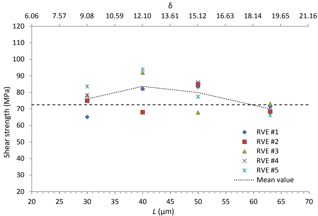
Fig.16 Transverse shear strength of RVEs with different sizes.
