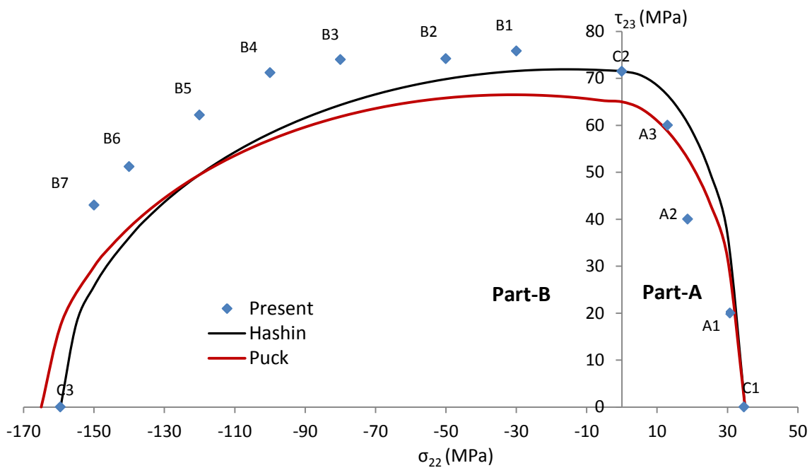
Fig.18 Failure envelope of a fibre-reinforced composite lamina in the \sigma_{22} - \tau_{23} stress space.
