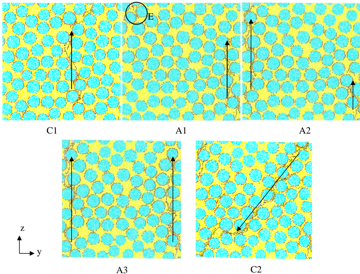
Fig.19 Accumulation of damages in the composite under different loading combinations in Part-A. (Each subfigure represents a data point on the failure envelope according to its label; Red dots represent fibre/matrix debonding and black dots represent matrix cracks.)
