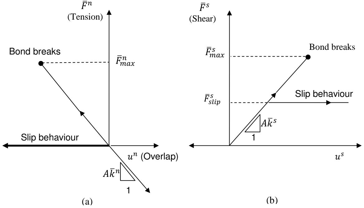
Fig.2 Force-displacement laws of parallel bond model: (a) normal behaviour, and (b) shear behaviour.
