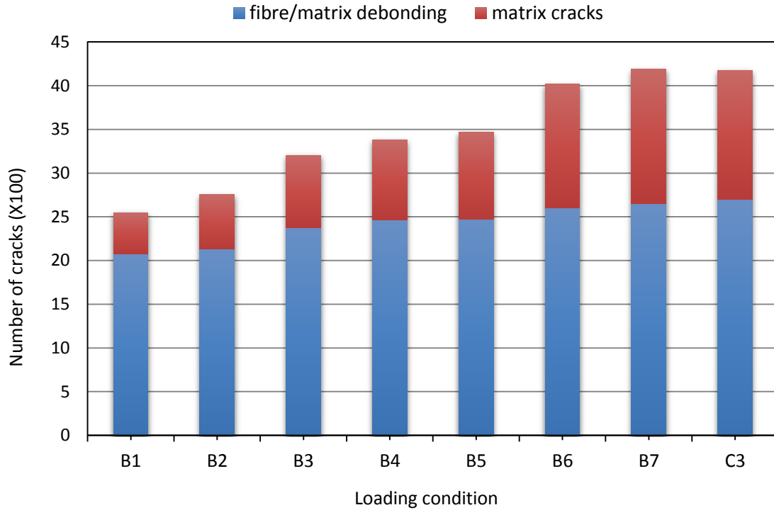
Fig.22 Number of fibre/matrix debonding and matrix cracks in loading cases in Part-B.
