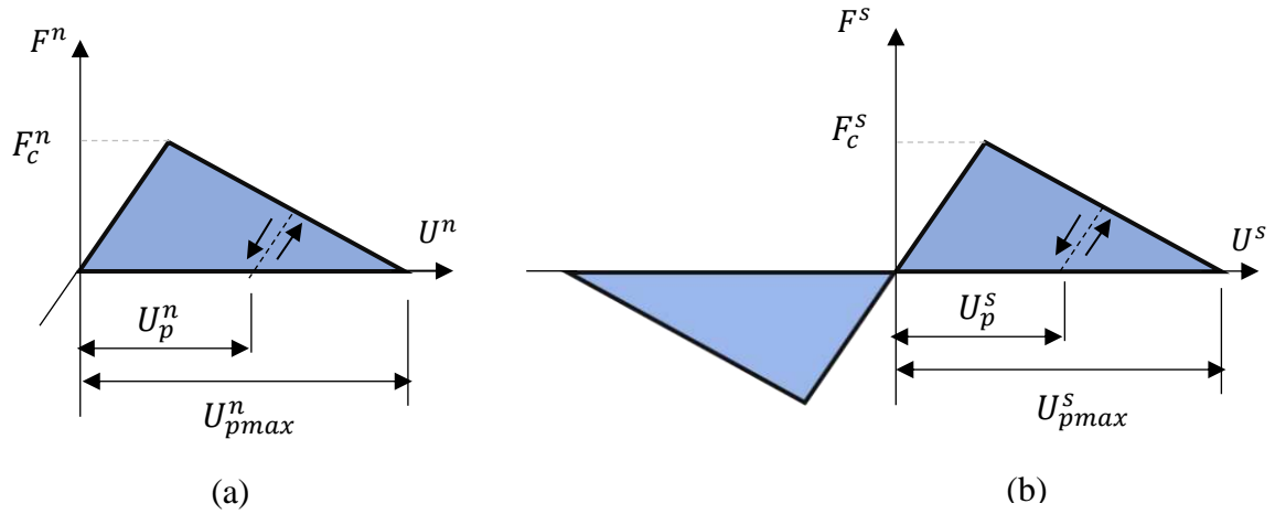
Fig.3 Constitutive behaviour of contact displacement-softening model: (a) normal behaviour, and (b) shear behaviour.
