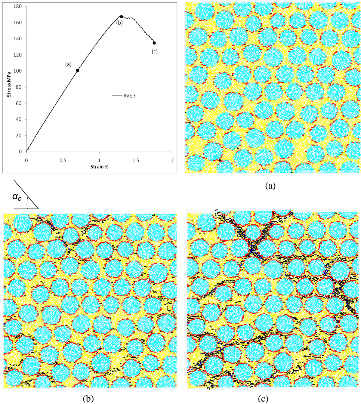
Fig.12 Damage evolution under transverse compression at different loading strains: (a) 0.7% (b) 1.3% (c) 1.7%. (Red dots are fibre/matrix debonding and black dots are matrix cracks)
