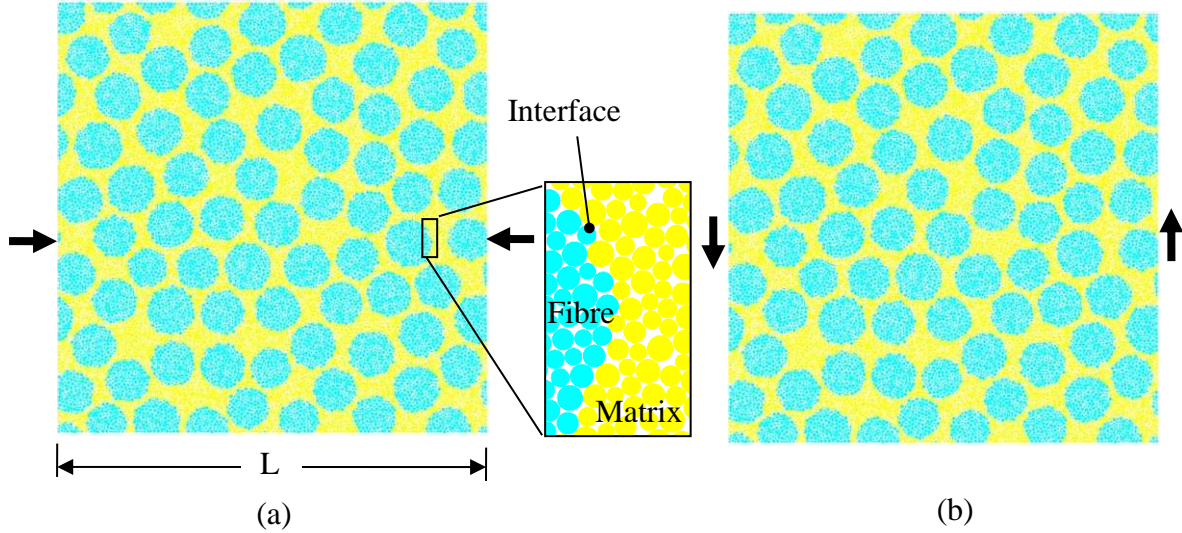
Fig.8 A RVE of DEM model subjected to: (a) transverse compression and (b) transverse shear (arrows indicate the loading directions).
