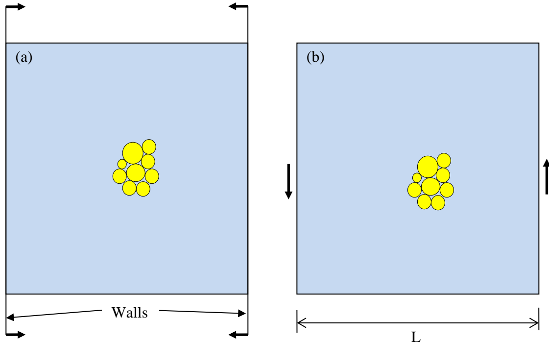
Fig.5 Virtual uniaxial tests of a DEM model: (a) compression and (b) shear.
