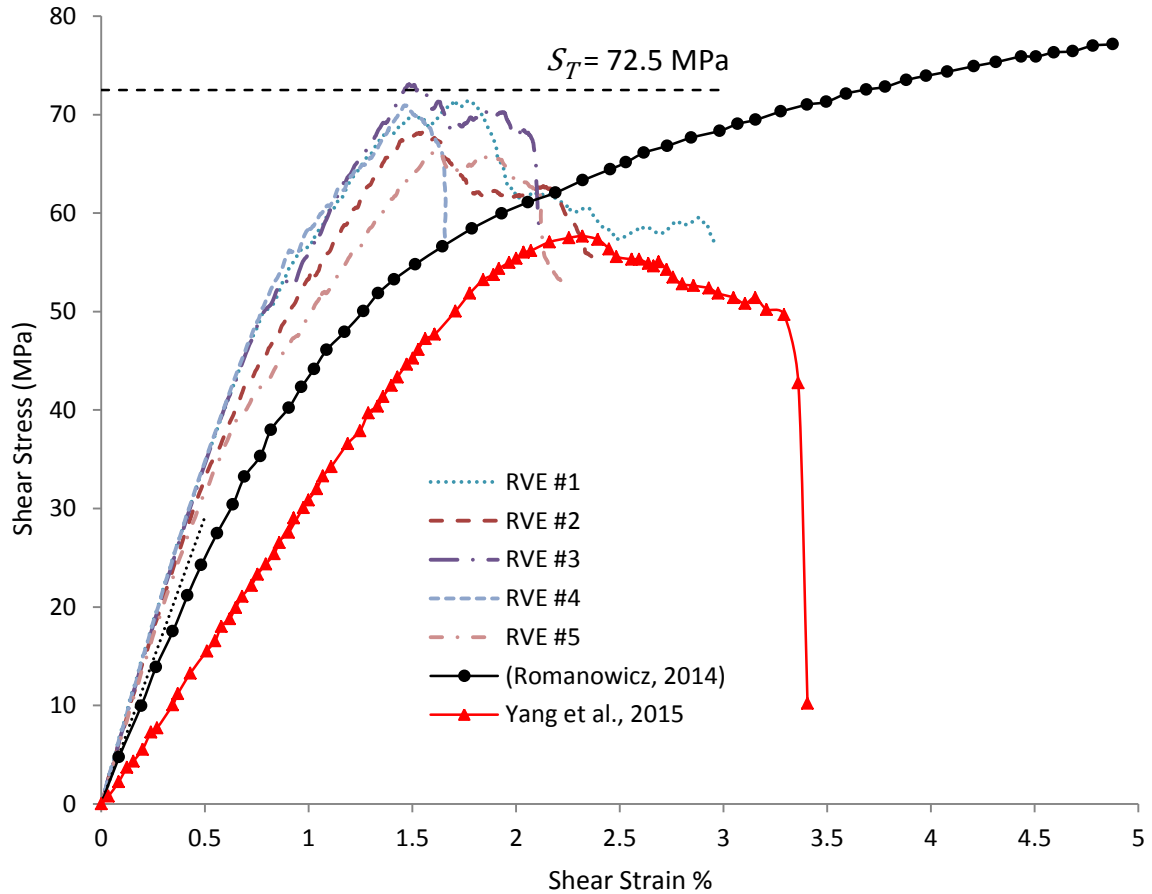
Fig.13 Transverse shear stress-strain curve using five different fibre arrangements compared with [19] and [41].
