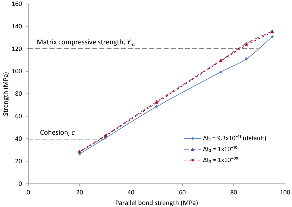
Fig.7 Influence of bond strength and time step on the macro compressive strength of a DEM model.
