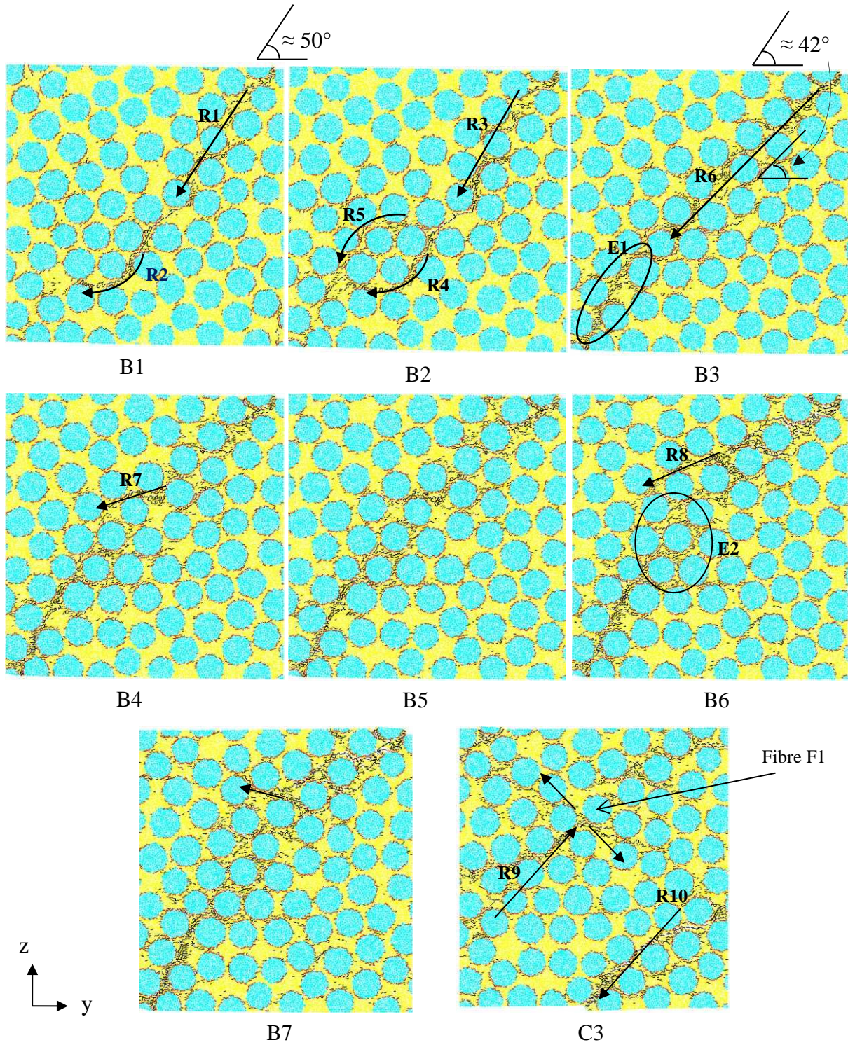
Fig.20 Accumulated cracks in the composite under different loading combinations. (Each subfigure represents a data point on the failure envelope according to its label; Red dots represent fibre/matrix debonding and black dots represent matrix cracks.)
