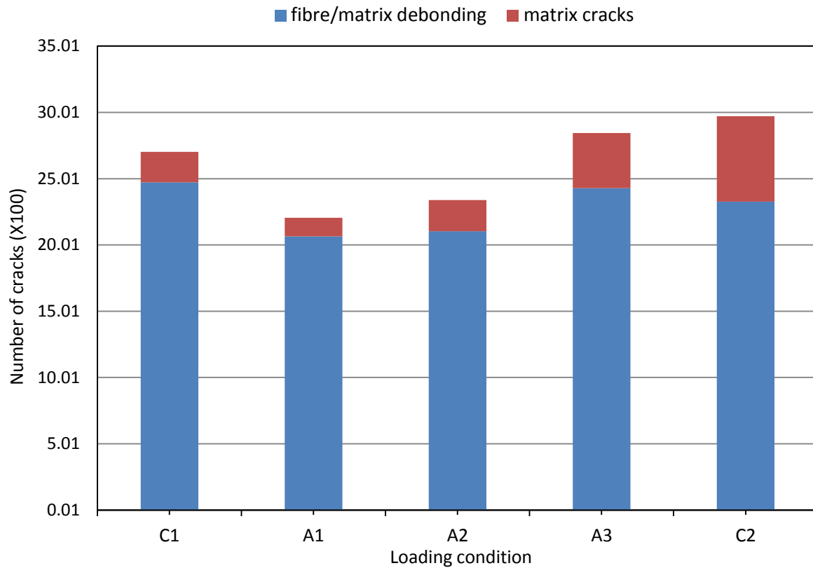
Fig.21 Number of fibre/matrix debonding and matrix cracks in loading cases in Part-A.
