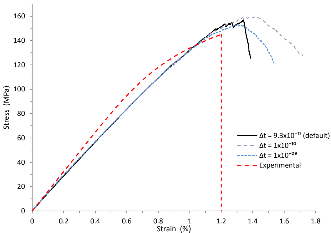
Fig.10 Stress-strain curves from DEM simulations using different time steps compared to experimental results [33].
