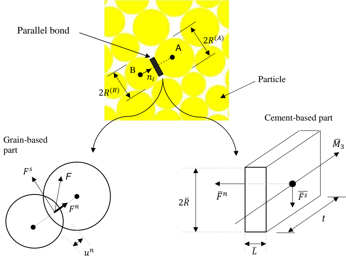
Fig.1 Schematic diagram of the parallel bond.
