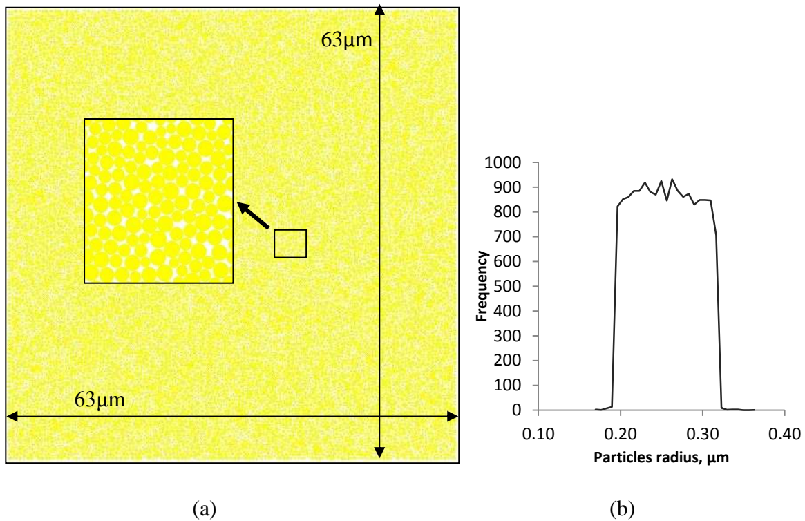
Fig.4 The DEM model: (a) model geometry and particle assembly, and (b) particle size distribution.
