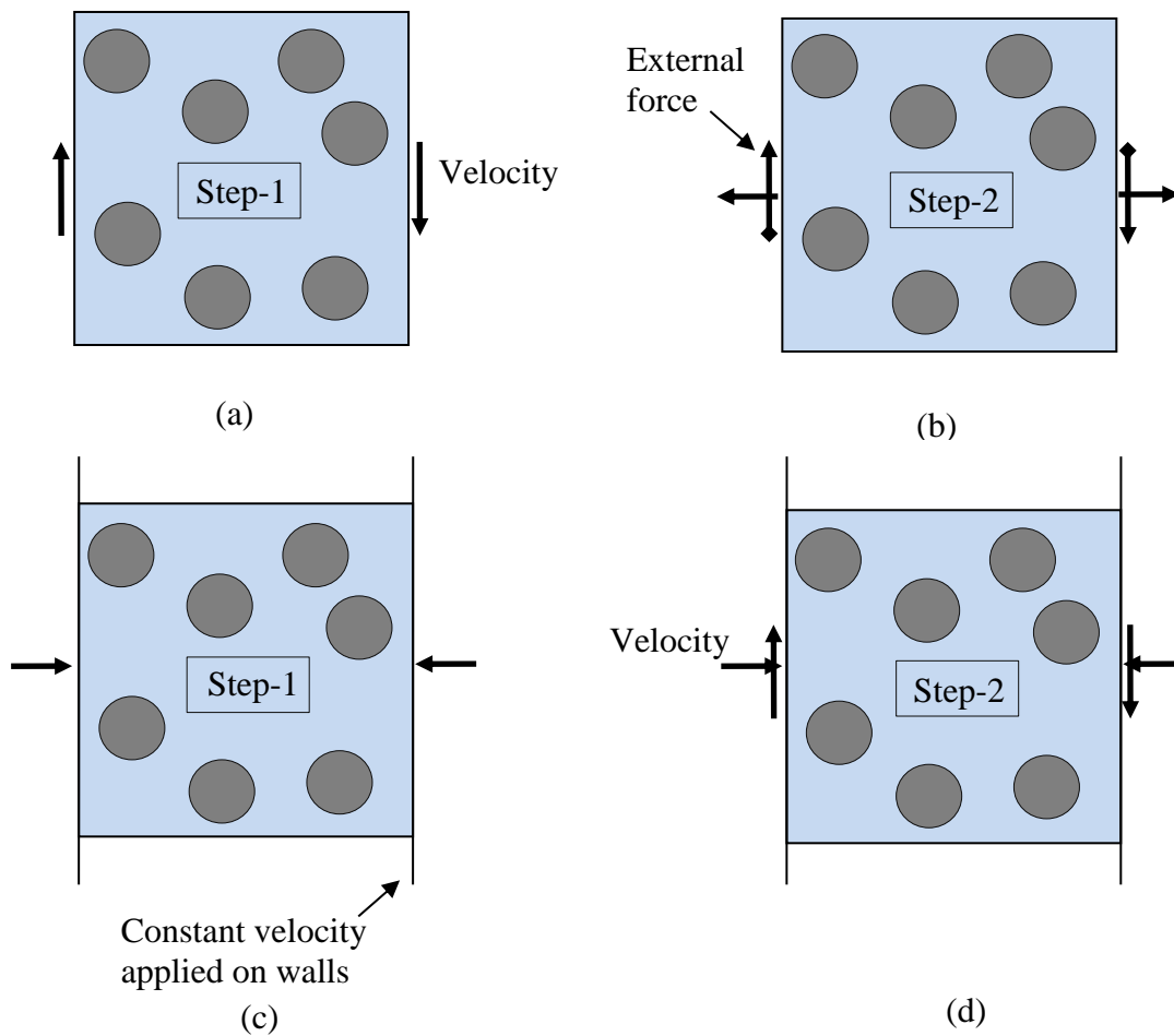
Fig.17 Loading schemes used to perform biaxial tests (arrows \blacktriangleleft\blacktriangleright represent external force and arrows \rightarrow represent velocity applied): (a)-(b) shear and tension in Part-A, and (c)-(d) shear and compression in Part-B.
