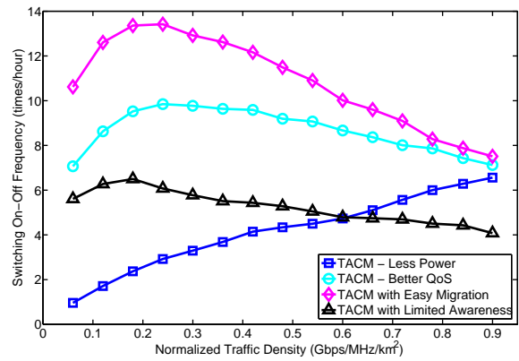
Fig. 10. Comparisons of the different versions of the TACM algorithm on the switching on-off frequency.
