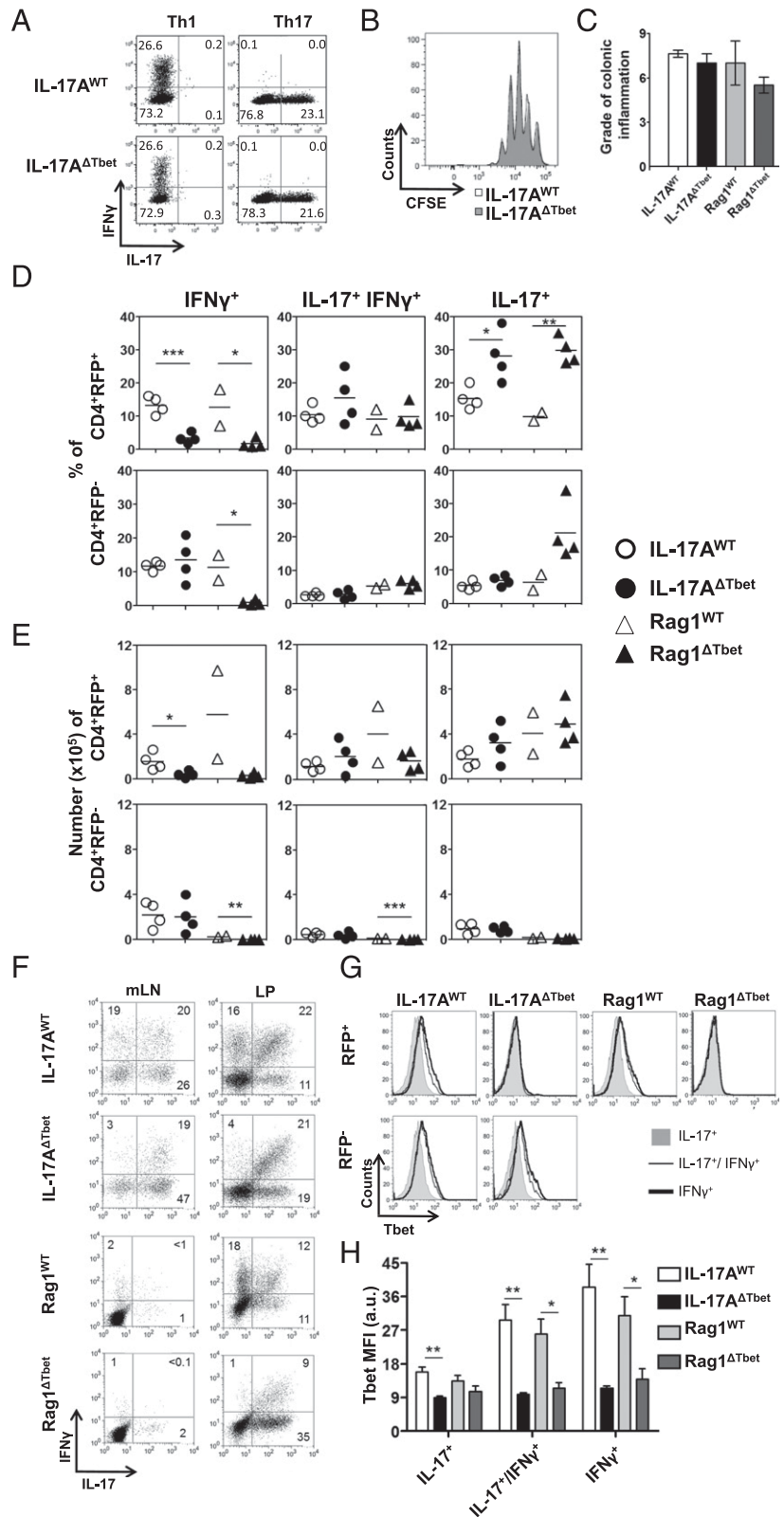
FIGURE 2. Th17 to Th1 conversion is not required for H. hepaticus -induced intestinal pathology. IL-17A WT mice were crossed with floxed Tbx21 mice and their naive T cell polarization potential assessed in vitro ( A and B ), and IL-17A WT , IL-17A ΔTbet , Rag1 WT , and Rag1 ΔTbet mice were inoculated with H. hepaticus ( Hh ) plus anti-IL-10R, and, 2 wk later, ceca, colons, and mLN were collected and processed for histology ( C ) and/or intracellular staining for cytokines and Tbet ( D–H ). (A) In vitro differentiation of naive CD4 + T cells from IL-17A WT controls and IL-17A ΔTbet mice toward Th1 and Th17 lineages. (B) Proliferation profile of naive CD4 + T cells cultured under Th17-polarizing conditions from indicated mouse lines. (C) Histology scores of ascending colon from indicated mouse lines 2 wk post- Hh /anti-IL-10R administration ( n = 4 per group except for Rag1 WT where only two mice were examined). Data for IL-17A WT and IL-17A ΔTbet mice are representative of two independent experiments. (D and E) Proportions (D) and numbers (E) of LP RFP + CD4 + and RFP - CD4 + T cells expressing IFN- \gamma alone, IL-17 alone, or both IFN- \gamma and IL-17 from pooled cecum and colon from indicated mouse lines 2 wk post- Hh /anti-IL-10R administration. Data for IL-17A WT and IL-17A ΔTbet mice are representative of two independent experiments. (F) Dot plots show the proportions of IL-17 single-positive, IL-17/IFN- \gamma double-positive, and IFN- \gamma single-positive cells within the mLN and LP RFP + CD4 + T cell population from indicated mouse lines 2 wk post- Hh /anti-IL-10R administration. (G) Assessment of Tbet expression by flow cytometry staining in RFP + (top row) or RFP - (bottom row) LP CD4 + T cells positive for either IL-17 alone (filled gray), IL-17 and IFN- \gamma (thin line), or IFN- \gamma alone (bold line) from indicated mouse lines 2 wk post- Hh /anti-IL-10R administration. (H) Average mean fluorescence intensity (MFI) of Tbet staining of indicated RFP + CD4 + T cell subsets derived from indicated mouse lines. Data are from the mice shown in (D) and (E) (averages \pm SEM). * p < 0.05, ** p < 0.01, *** p < 0.001.
