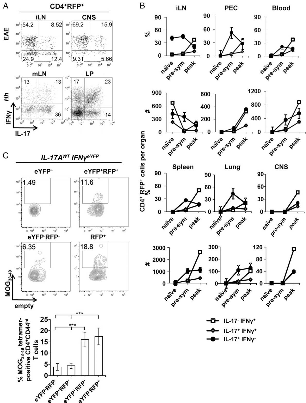
FIGURE 1. The Th17 cell lineage dominates during inflammation. IL-17A fate-reporter mice (IL-17A WT ) were subjected to MOG/CFA administration to induce EAE or given H. hepaticus ( Hh ) plus anti-IL-10R mAb to induce typhlocolitis, and the cytokine-secreting phenotype of Th17 lineage-positive (RFP + ) CD4 + cells was assessed at different time points. (A) Representative intracellular flow cytometry plots for IFN- \gamma and IL-17 of gated RFP + CD4 + T cells during EAE (day 17) in iLN and CNS, or during H. hepaticus colitis (day 14) in mLN and large intestinal LP. (B) Dynamics of Th17 cell-derived populations as a proportion of RFP + CD4 + T cells ( upper panels ) and their absolute numbers ( lower panels ) in indicated tissues during EAE induction (PEC, peritoneal exudate cells). Naïve = prior to MOG/CFA administration, presym = presymptomatic (day 6), and peak = peak of clinical score (day 17). Values represent average \pm SEM, n = 4 /time point. (C) Representative staining for I-Ab/MOG 38-49 ( top flow panels ) and average distribution ( bottom panel ) in indicated T cell populations as proportion of CD4 + CD44 hi T cells harvested from the CNS of IL-17A WT IFN- \gamma eYFP mice at day 17 after EAE induction. Data are representative of two independent experiments (average \pm SEM, n = 6 ), *** p < 0.001 .
