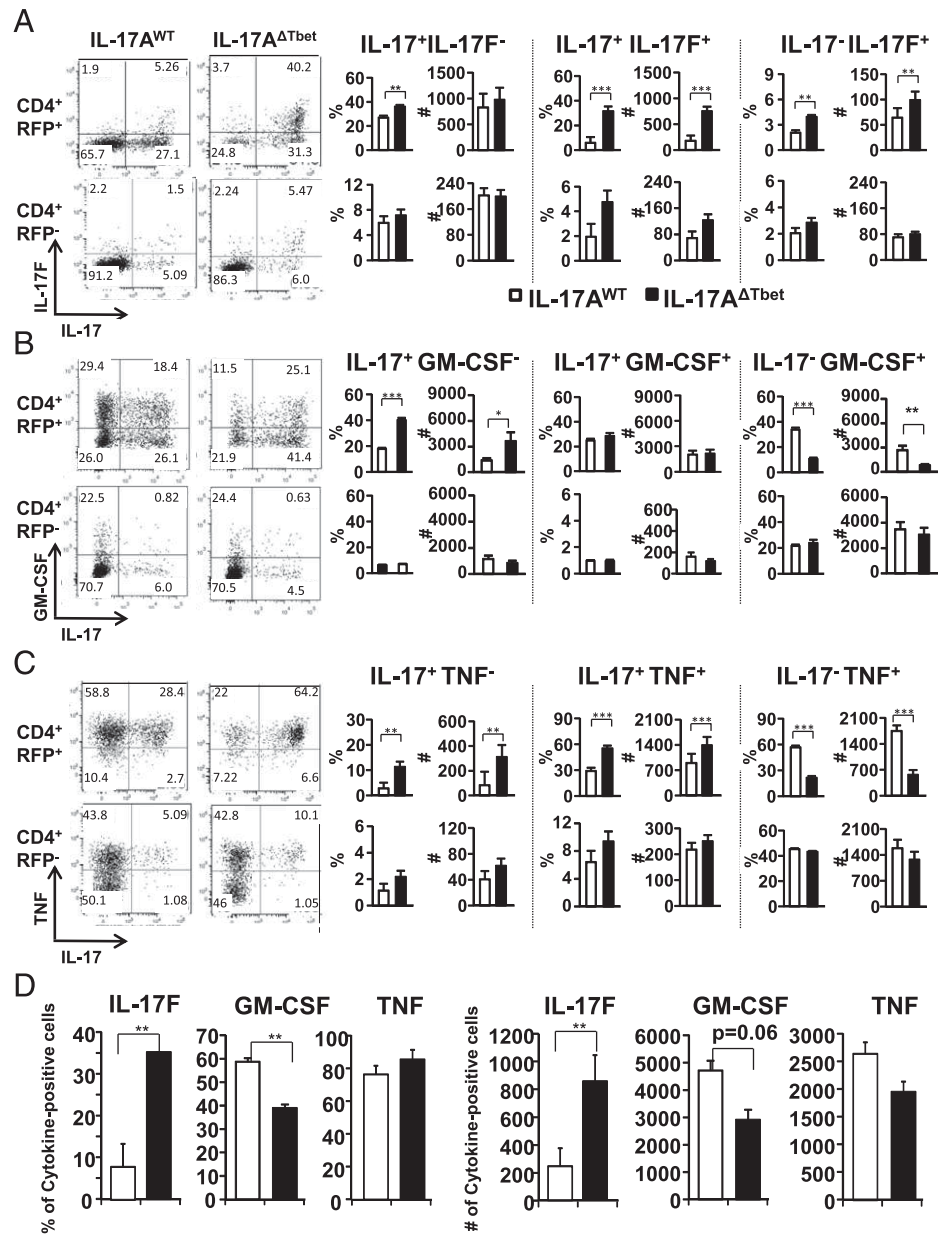
FIGURE 4. Characterization of Tbet-deficient Th17 cells in EAE. T cells were sourced from the CNS of IL-17A WT controls and IL-17A ΔTbet mice at the peak of EAE symptoms (day 15–17) and characterized for their cytokine production (A–D). RFP + Th17 lineage-positive (top panels) and RFP - lineage-negative (bottom panels) cells from IL-17A WT controls (white bars) or IL-17A ΔTbet mice (black bars) were stained for IL-17, GM-CSF, and TNF, and proportions (left panels) and cell numbers (right panels) of cells expressing IL-17 and/or IL-17F (A), GM-CSF (B), and TNF (C) are shown. (D) Total proportion and numbers of IL-17F - , GM-CSF - , and TNF-producing CD4 + T cells present in the CNS of indicated mouse lines (averages ± SEM, n = 4–5). *p < 0.05, **p < 0.01, ***p < 0.001.
