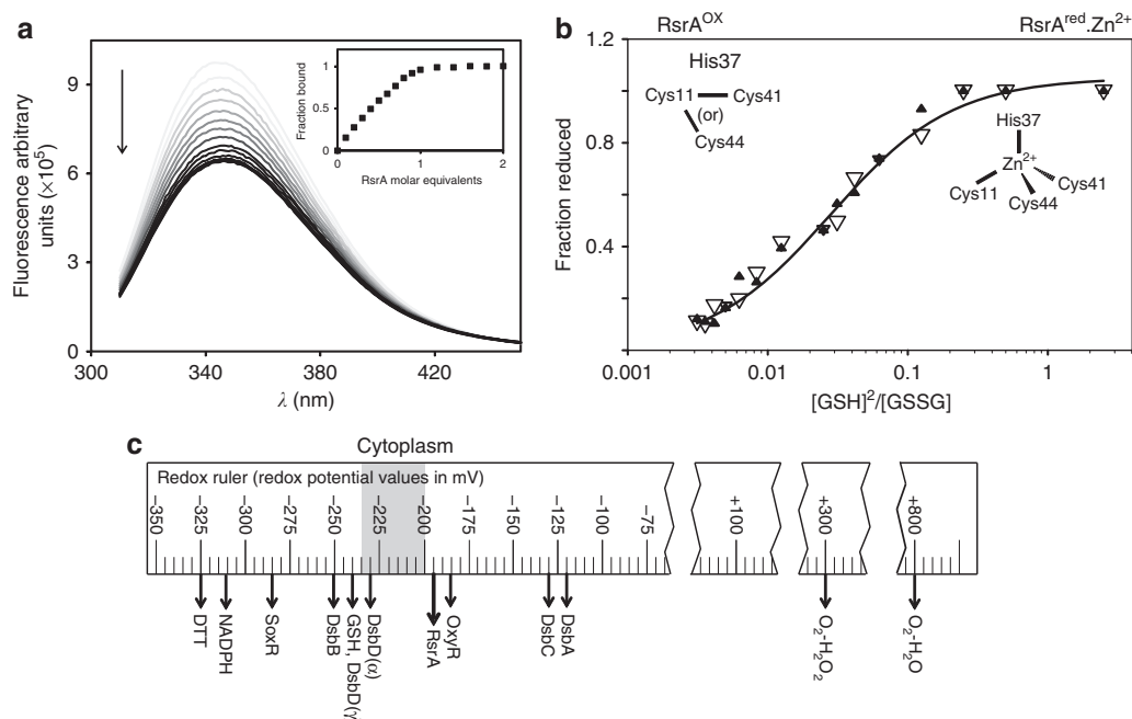
Figure 2 | Redox potential of the RsrA^{red}.Zn^{2+}-\sigma^R complex. (a) RsrA^{red}.Zn^{2+} binding to \sigma^R monitored by intrinsic tryptophan emission fluorescence spectroscopy. Figure shows emission spectra ( \lambda_{ex} 295 nm) of \sigma^R at different RsrA^{red}.Zn^{2+} concentrations collected at 25 °C in 50 mM Tris (pH 7.5) buffer, 100 mM NaCl and 2 mM DTT. For clarity, traces are coloured with incrementally darker tone of grey for increasing RsrA concentration. Inset figure shows fraction of \sigma^R in complex as measured by the change in fluorescence intensity at 343 nm with increasing RsrA^{red}.Zn^{2+} concentration. Data show stoichiometric binding of RsrA^{red}.Zn^{2+} to \sigma^R . (b) Redox potential of RsrA^{red}.Zn^{2+} in complex with \sigma^R complex relative to a redox couple of reduced/oxidized glutathione. The degree of oxidation was measured by the change in tryptophan emission fluorescence of \sigma^R as the complex dissociates (open triangles) and by the release of Zn^{2+} using the PAR assay (filled triangles). Both sets of data were fitted to the Nernst equation to determine the redox potential of the RsrA^{red}.Zn^{2+}-\sigma^R complex as -193.04 \pm 2.01 mV. Experiments were conducted in 50 mM Tris (pH 7.5) buffer containing 100 mM NaCl and at 25 °C. (c) Redox ruler showing the redox potentials of selected proteins and small molecules. Figure adapted from ref. 27. The estimated redox potential of the bacterial cytoplasm is indicated in grey.
