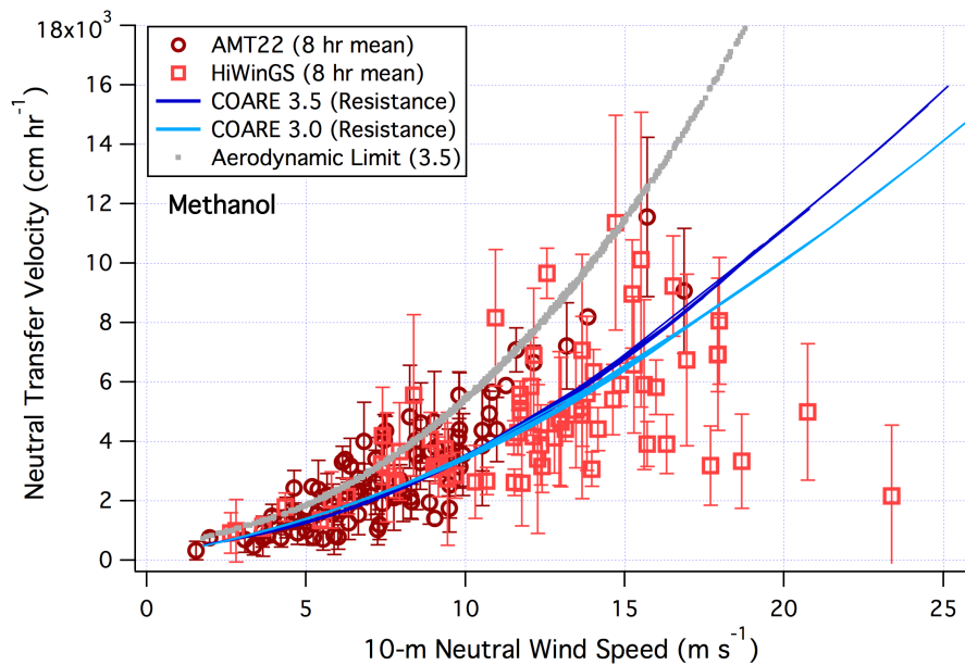
Figure 4. Transfer velocity of methanol from AMT-22 and HiWinGS cruises.
