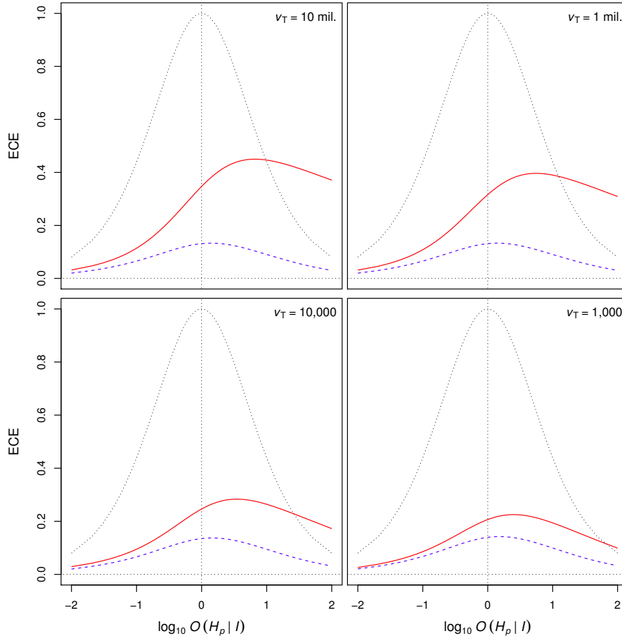
Figure 9: ECE plots from a simulation study with different thresholds v_T on V . The solid curves represent the accuracy; the dashed curves the calibrated accuracy; and the dotted curves the neutral reference. The x-axis is \log_{10} of the prior odds in favour of H_p , that is O(H_p|I) = \Pr(H_p|I)/\Pr(H_d|I) .
