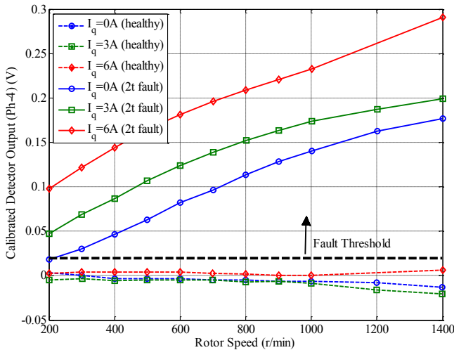
Fig. 21: Variation of calibrated detector output (ph-4) at various loading (0%, 50%, 100%) with varying speed. Dashed curves refer to healthy motor operation and solid lines refer to 2-turn fault condition.
