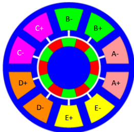
Fig. 1: Geometry of 10-slot, 12-pole SPM machine
