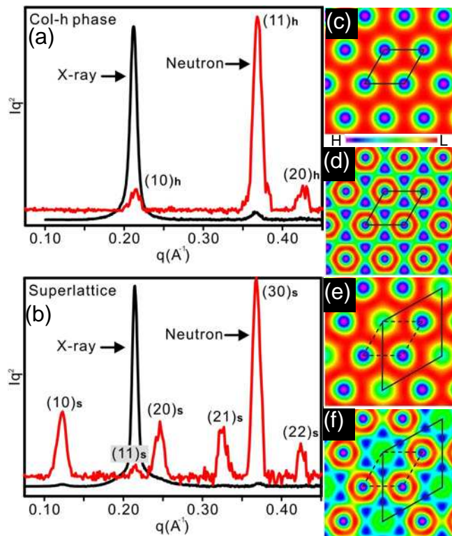
Figure 2. (a,b) Small-angle X-ray (black) and neutron powder diffractograms (red) of 12-12-12Li + C 19 D 40 80/20 in the (a) Col h phase at 70 °C and (b) the superlattice phase at 130 °C. (c) ED and (d) neutron SLD map of the Col h phase. (e) ED and (f) SLD map of the Col s . Neutron experiments at station D16 at ILL, Grenoble.
