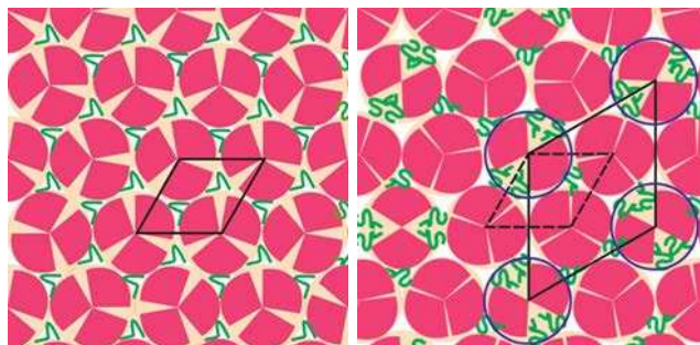
Figure 3. Schematic model of a layer of the 12-12-12Li + C 19 D 40 80/20 blend in the (a) Col h and (b) superlattice phase (pink: minidendrons; green: n-alkane).
