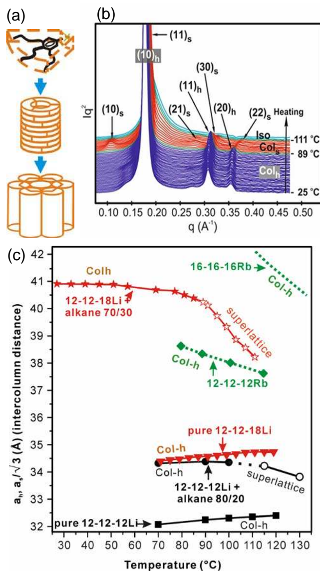
Figure 1. (a) Self-assembly of dendrons in a columnar phase (schematic). (b) SAXS curves for 12-12-18Li + C 19 D 40 70/30 recorded during first heating. SAXS experiments were done at beamline I22 at Diamond, UK. (c) Temperature dependence of intercolumnar distance in Col h and Col s phases of 12-12-12Rb , 12-12-12Li , 12-12-18Li , 12-12-12Li + C 19 D 40 80/20 and 12-12-18Li + C 19 D 40 70/30. The trendline for 16-16-16Rb from ref. 9 is also added.
