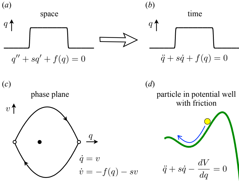
FIGURE 37. The main ideas of spatial dynamics. The steady spatial problem (a) is viewed as second-order equation in time (b). From this its solutions may be analysed in the phase plane (c) or using a mechanical analogy (d).
