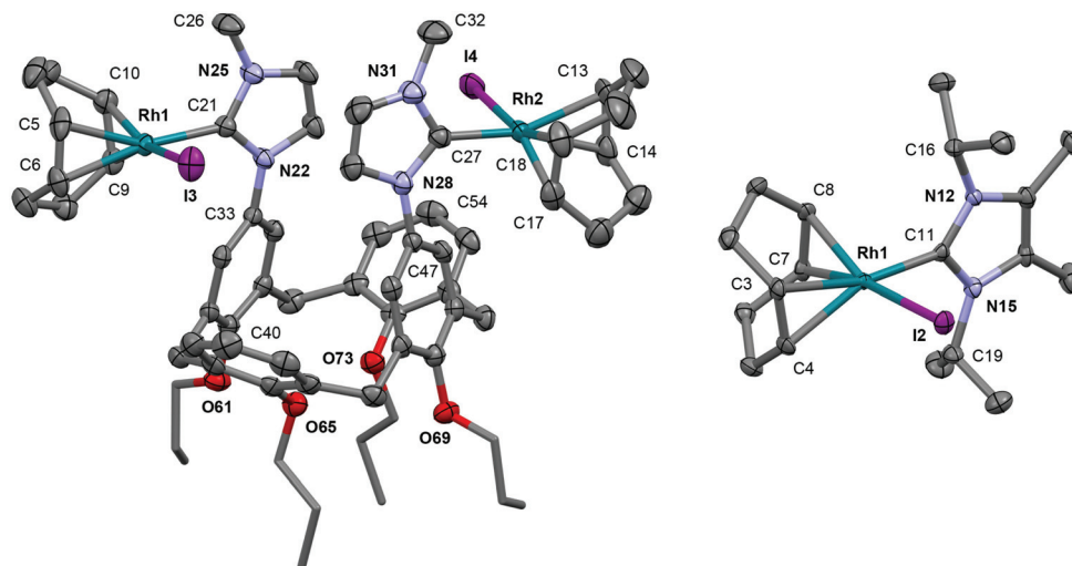
Fig. 2 Solid-state structures of 2a and 2b . Thermal ellipsoids for selected atoms drawn at the 50% probability level; minor disordered components (two O n Pr groups in 2a ), and hydrogen atoms omitted for clarity. Selected bond lengths (Å) and angles (°): 2a : Rh1–I3, 2.6905(3); Rh1–Cnt(C5,C6), 2.089(3); Rh1–Cnt(C9,C10), 2.001(3); Rh1–C21, 2.021(3); Rh2–I4, 2.6934(3); Rh2–Cnt(C13,C14), 2.098(3); Rh1–Cnt(C17,C18), 1.990(4); Rh2–C27, 2.024(3); Rh1...Rh2, 8.5698(3); Cnt(C21–N25)–Cnt(C27–N31), 3.608(5); ∠Mpln(C33–C38,O61)–Mpln(C47–C52,O69), 22.35(6); ∠Mpln(C40–C45,O65)–Mpln(C54–C59,O73), 76.06(6); 2b : Rh1–I2, 2.6729(2); Rh1–Cnt(C3,C4), 2.109(2); Rh1–Cnt(C7,C8), 2.00(3); Rh1–C11, 2.021(3).
