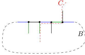
Figure 33: The crossing cycles in the proof of (60).
