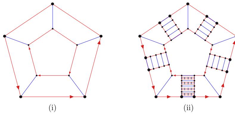
Figure 2: A twist-squeeze-amalgamation.
