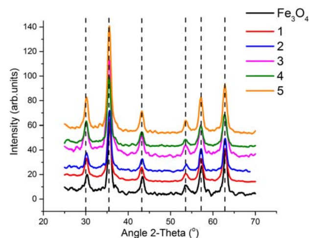
Figure 1. XRD patterns of non-stabilised \text{Fe}_3\text{O}_4 and heparin-stabilised \text{Fe}_3\text{O}_4 nanoparticles prepared according to Table 1. Dashed lines represent expected peak positions for cubic magnetite according to the JCPDS database.
