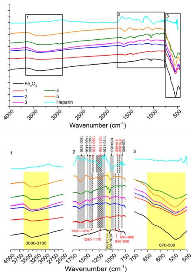
Figure 3. IR spectra of non-stabilised \text{Fe}_3\text{O}_4 nanoparticles, heparin and heparin-stabilised \text{Fe}_3\text{O}_4 nanoparticles, prepared according to Table 1, as labelled (top). Black squares are zoomed in (bottom, as labelled) with stretches labelled and highlighted: yellow for stretches associated with \text{Fe}_3\text{O}_4 , grey for those associated with heparin, with shifted stretches due to association of heparin with particles highlighted by striped grey bars and red text.
