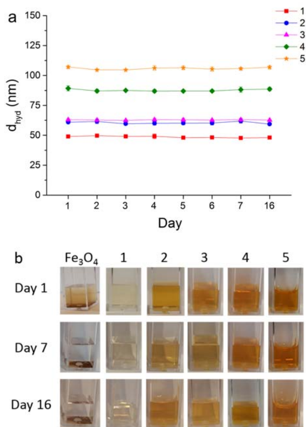
Figure 6. a) Hydrodynamic diameters ( d_{\text{hyd}} ) of heparin-stabilised \text{Fe}_3\text{O}_4 nanoparticles, prepared according to Table 1, recorded over several days showing negligible changes in size; b) Photographs of samples over several days illustrating precipitation of non-stabilised \text{Fe}_3\text{O}_4 and stability of heparin-stabilised samples, as labelled.
