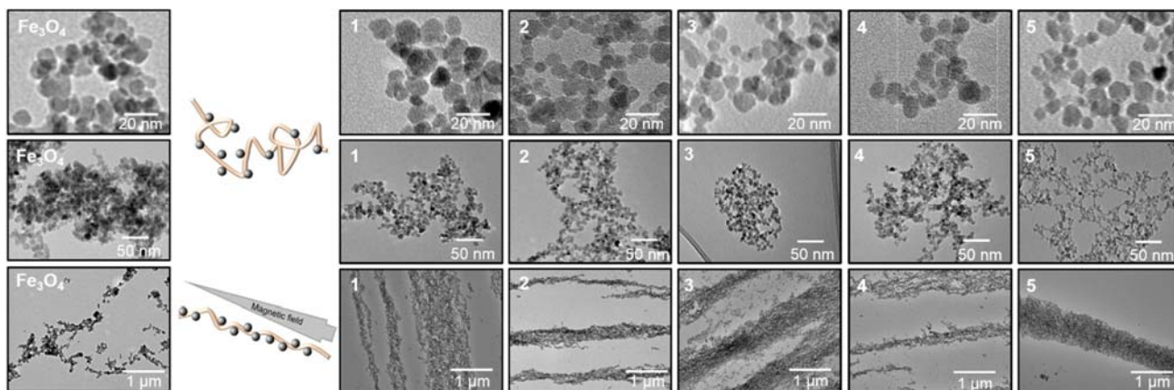
Figure 5. Transmission electron microscope (TEM) images of non-stabilised \text{Fe}_3\text{O}_4 and heparin-stabilised \text{Fe}_3\text{O}_4 nanoparticles, labelled as prepared according to Table 1. Top row: images taken in the absence of a magnetic field at high magnification. Middle row: images taken in the absence of a magnetic field at low magnification. Bottom row: images taken in the presence of a parallel permanent magnetic field at low magnification. Schematics represent the behaviour of stabilised \text{Fe}_3\text{O}_4 particles in the absence and presence of a parallel magnetic field.
