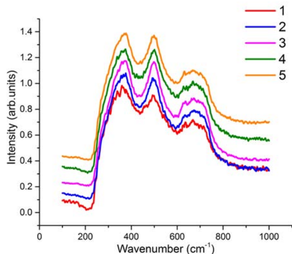
Figure 2. Raman spectra of heparin-stabilised \text{Fe}_3\text{O}_4 nanoparticles prepared according to Table 1.
