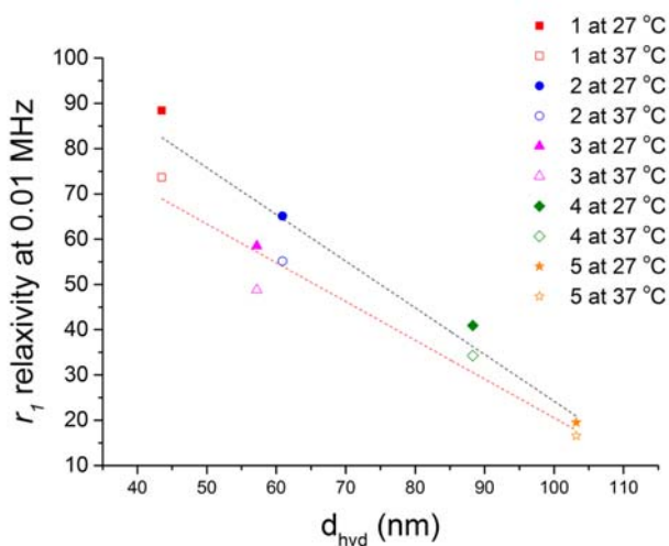
Figure 8. Low frequency relaxivity ( r_1 at 0.01 MHz at 27 °C (filled symbols) and 37 °C (open symbols)) of heparin-stabilised \text{Fe}_3\text{O}_4 nanoparticles plotted as a function of hydrodynamic diameter ( d_{\text{hyd}} ). Dotted lines represent a linear fit of data collected at 27 °C (black) and 37 °C (red).
