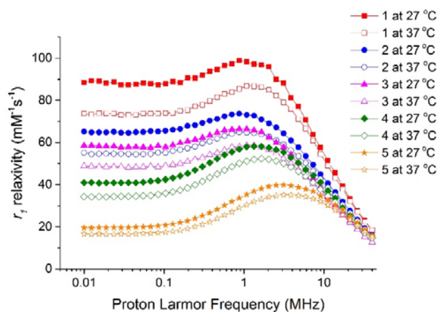
Figure 7. ^1\text{H} NMRD profiles for heparin-stabilised \text{Fe}_3\text{O}_4 nanoparticles, prepared according to Table 1. The r_1 values have been calculated in terms of [Fe] content of the samples. Profiles have been measured at two different temperatures, representative of room temperature (27 °C) and body temperature (37 °C).
