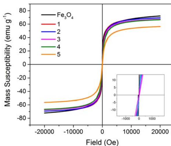
Figure 4. Magnetisation (mass susceptibility) versus field profiles of non-stabilised \text{Fe}_3\text{O}_4 and heparin-stabilised \text{Fe}_3\text{O}_4 nanoparticles, prepared according to Table 1.
