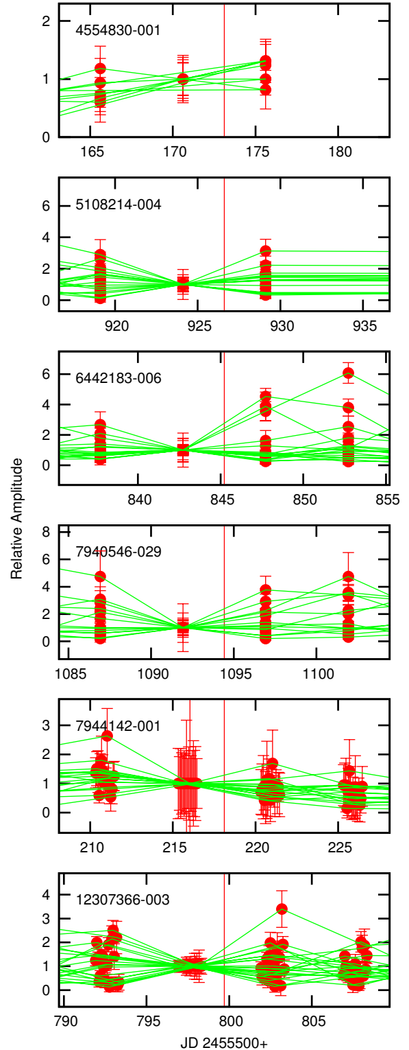
Figure 11. Pulsation amplitudes for solar-like oscillations as a function of time. The amplitudes have been normalized to the values just before the flare and one- \sigma error bars are shown. Solid lines join individual mode frequencies. The time of the flare is indicated by the vertical line.
