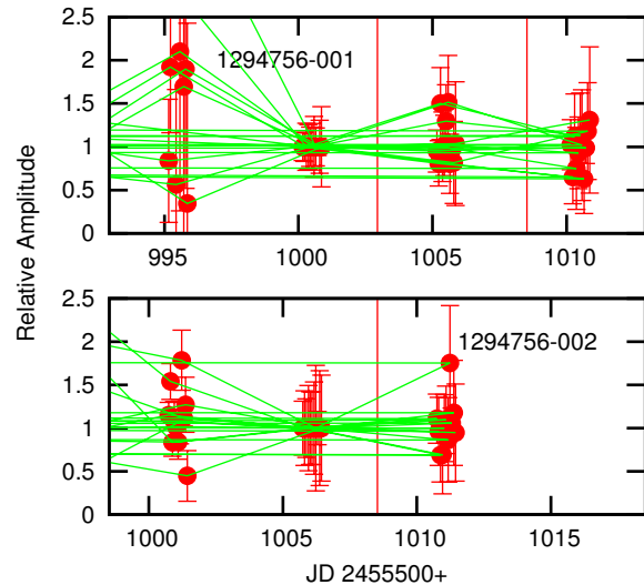
Figure 14. Relative pulsation amplitudes for the \delta Sct star KIC 1294756 as a function of time. The amplitudes have been normalized to the values just before the flare and one- \sigma error bars are shown. The time of the flare is indicated by the vertical line.
