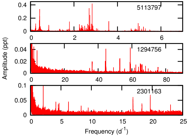
Figure 12. Periodograms of a \gamma Dor star (KIC 5113797, top panel) and two \delta Sct stars that show flares.
