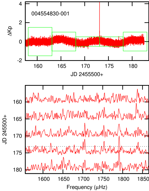
Figure 10. Top panel: light curve of KIC 4554830 showing flare and regions where periodograms were calculated. Bottom panel: periodograms of the regions shown in the top panel showing the solar-like oscillations. The dotted line shows the time of the flare.
