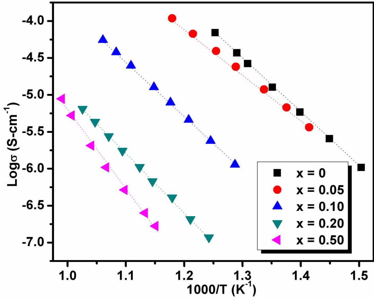
Fig. 7. Arrhenius plot of conductivity of (1-x)\text{BaTiO}_3-x\text{Bi}(\text{Mg}_{2/3}\text{Nb}_{1/3})\text{O}_3 ( x = 0-0.6 )
