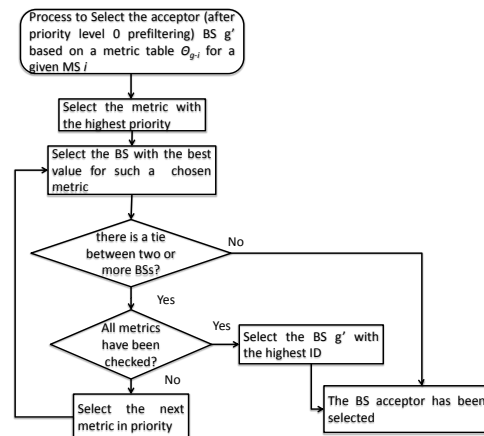
Figure 3. Flowchart of the sorting phase after pre-filtering in HHEA-DBC.
