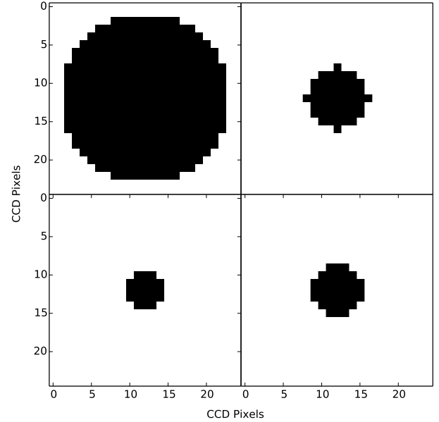
Fig. 1. Example apertures for (clockwise from top left) Kepler magnitude \leq 10 , \leq 13 , \leq 16 , > 16 .
