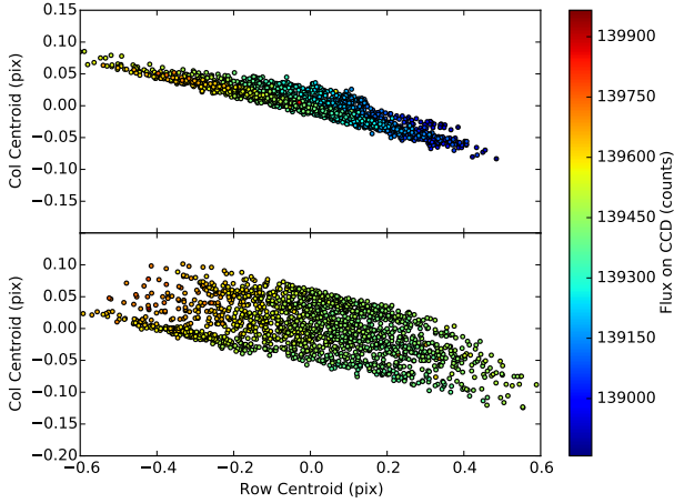
Fig. 2. Surface of raw flux against CCD position for EPIC201552917. The flux is split at 2016 (BJD-2 454 833), with the first segment above and the second segment below . Centroids have been offset to their respective means.
