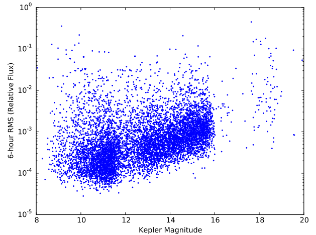
Fig. 6. Root median square plot of all (i.e. variable and non-variable) Campaign 0 detrended lightcurves binned into 6-h bins. A small random noise on the magnitudes has been added for clarity.
