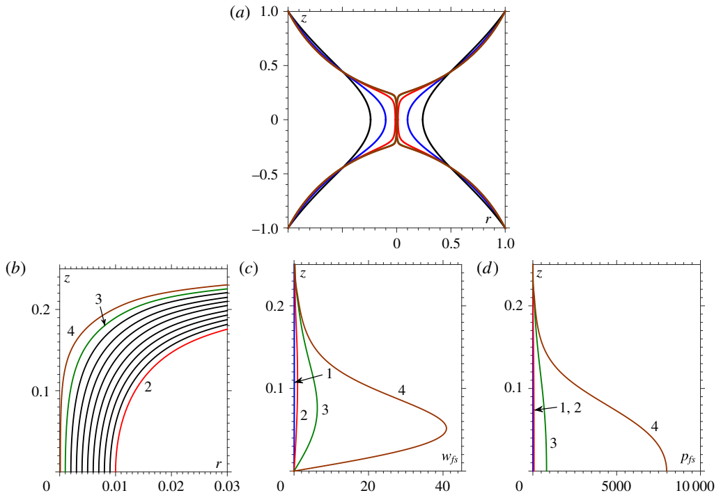
FIGURE 3. (Colour online) For Oh = 10 , characteristic of the V-regime, plots show (a) evolution of the entire free surface, (b) a close-up of the breakup region, (c) the axial velocity at the free surface, w_{fs} , and (d) the pressure at the free surface, p_{fs} , at r_{min} = 10^{-1} (1, blue), r_{min} = 10^{-2} (2, red), r_{min} = 10^{-3} (3, green) and r_{min} = 10^{-4} (4, brown).
