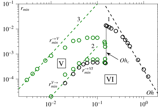
FIGURE 14. (Colour online) Phase diagram showing the low- Oh V-regime and the VI-regime. The transition r_{min}^{V \rightarrow VI} follows the scaling r_{min} = 2.3 \times 10^{-4} Oh^{-3.1} (curve 1) for Oh > Oh_c = 0.15 . For Oh < Oh_c the low- Oh V-regime appears and is bounded by curves 2: r_{min} = 0.2Oh^2 and 3: r_{min} = 10Oh^2 as r_{min} \rightarrow 0 .
