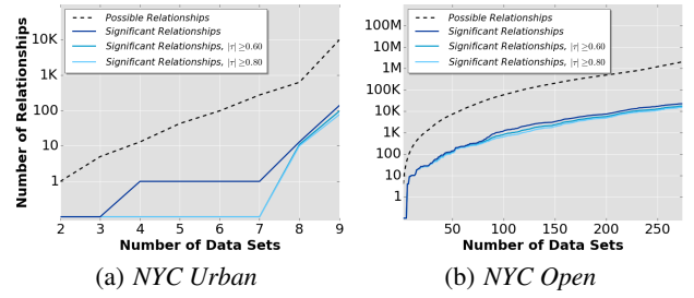
Figure 11: Relationship pruning.
