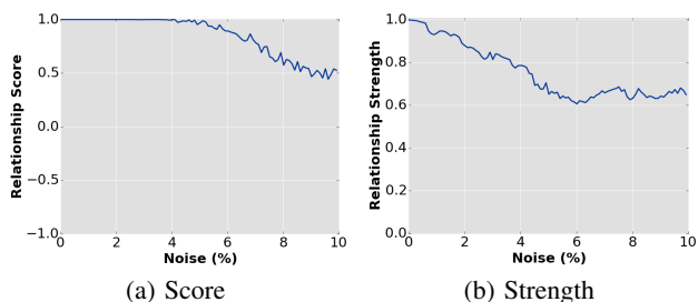
Figure III: Robustness evaluation (average of total taxi fare).
