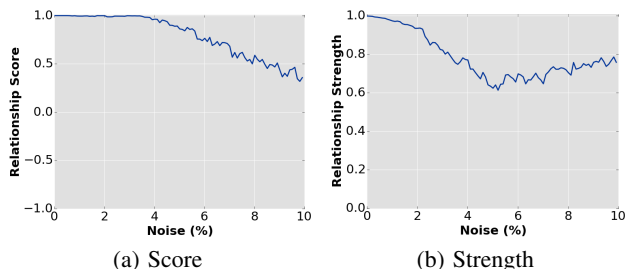
Figure II: Robustness evaluation (average of traveled miles).
