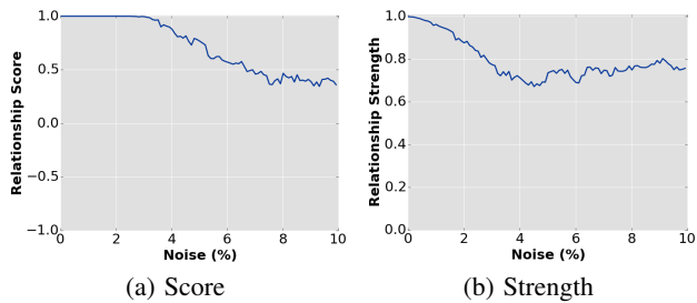
Figure I: Robustness evaluation (unique number of taxis).
