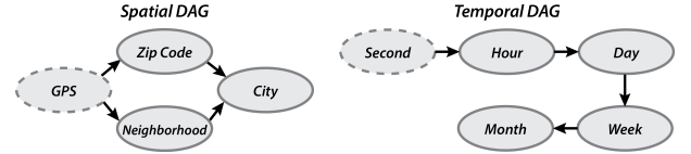
Figure 6: Hierarchical relationship for spatio-temporal resolutions represented by DAGs. Resolutions depicted using solid lines are used for evaluating relationships.
