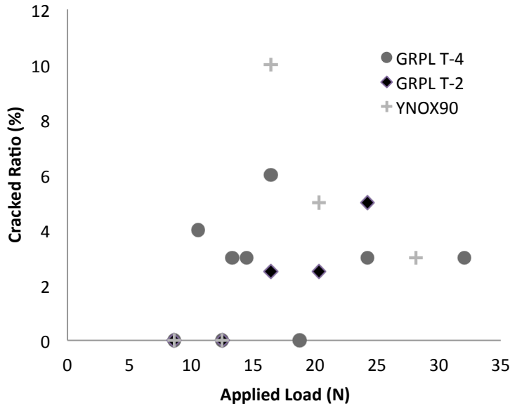
Figure 11 Graph showing proportion of broken grains for various loads and different rubber samples
