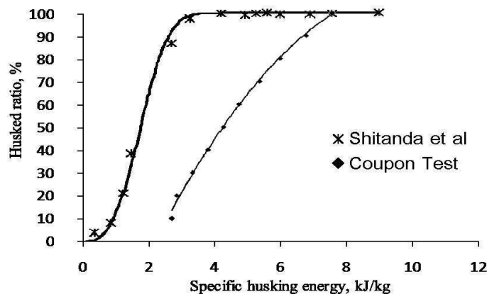
Figure 12 Plot of the rice husked ratio against specific husking energy.
