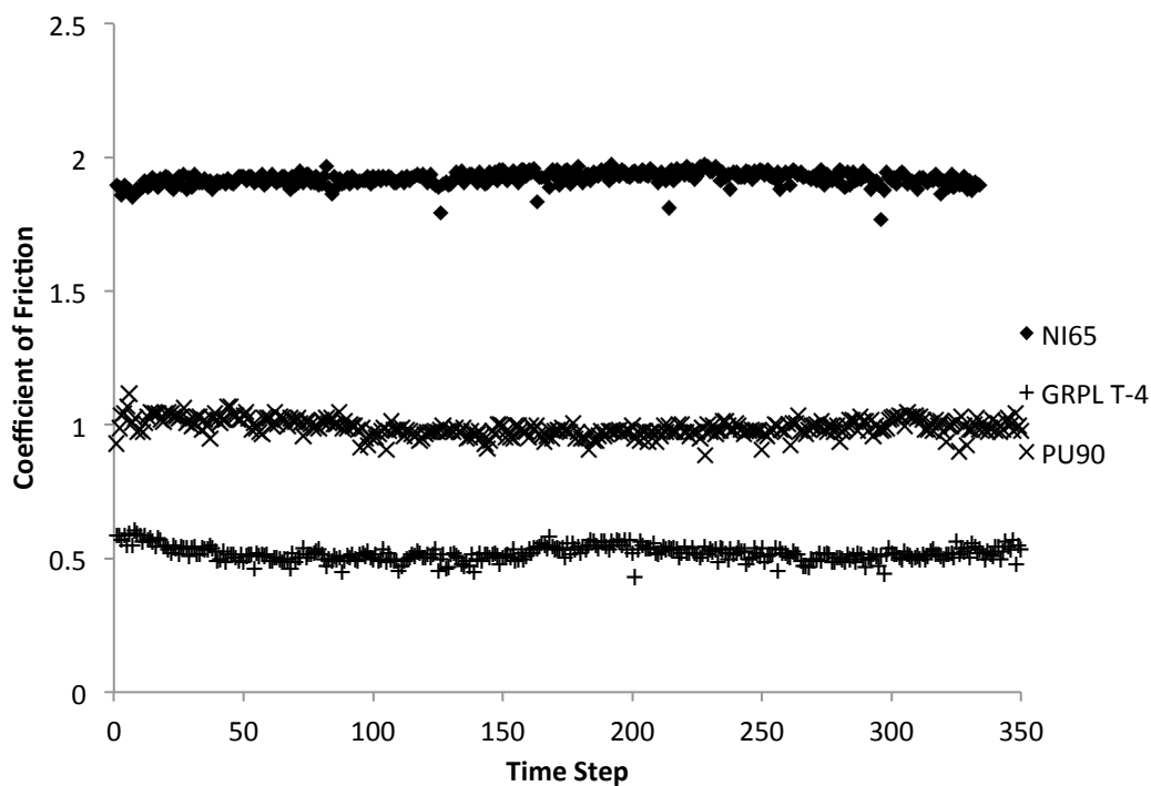
Figure 13 Coefficient of friction recorded as un-husked rice grains slide against for polyurethane samples.
