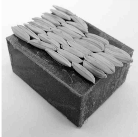
Figure 4 Block for friction test consisting of rice grains glued to a sample holder.
