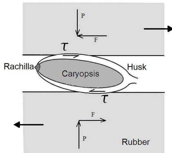
Figure 20 Schematic of the mechanism by which rice is husked between two rubber counterfaces
