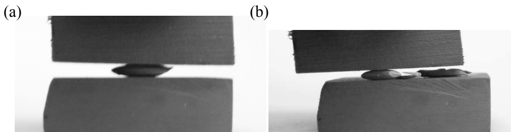
Figure 5 Stills extracted from high speed video footage of rubber samples with grain between, before (a) and after (b) husking
