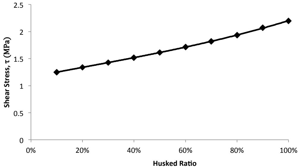
Figure 17 The mean limiting shear stress (assumed to be constant for each rubber sample) required to husk rice plotted against the ratio husked.
