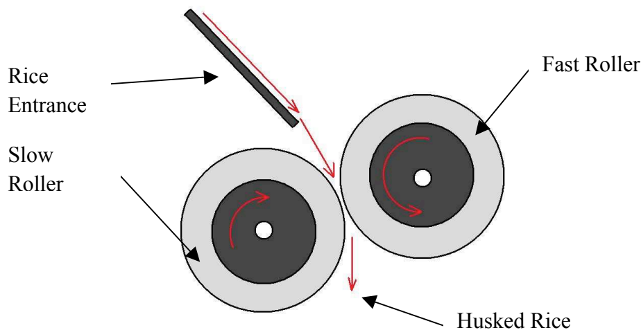
Figure 1 Schematic of Rubber Roll husker
