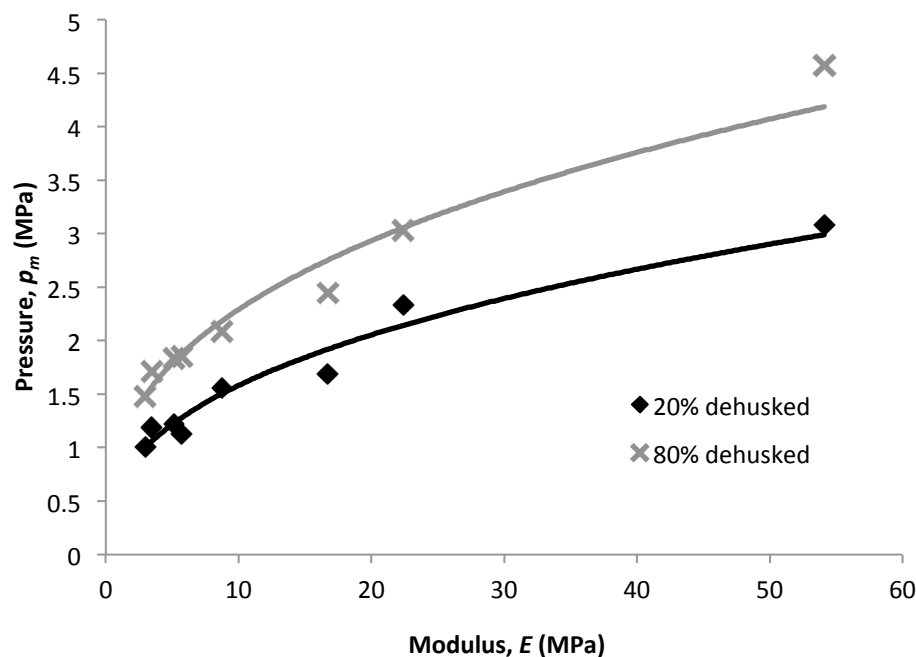
Figure 15 Mean contact pressure to achieve a 20% and 80% husked ratio plotted against the modulus of the rubber sample.
