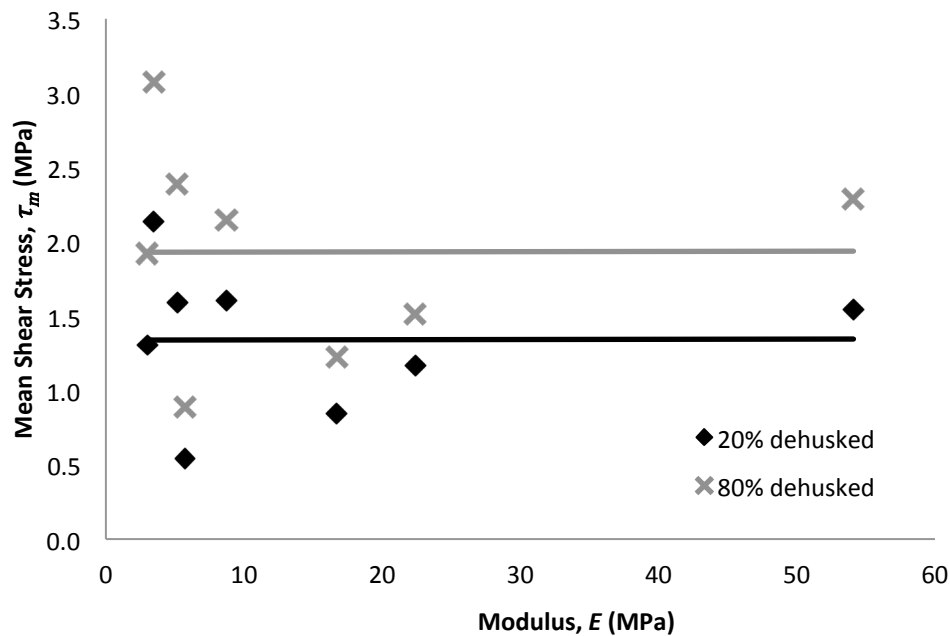
Figure 16 Mean shear stress to achieve a 20% and 80% husked ratio plotted against the modulus of the rubber sample.
