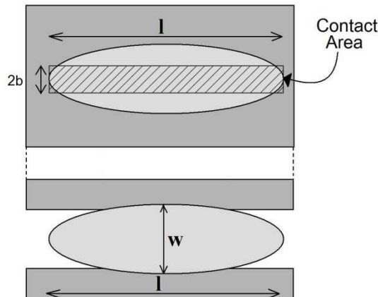
Figure 14 Hertz Line Contact Model
