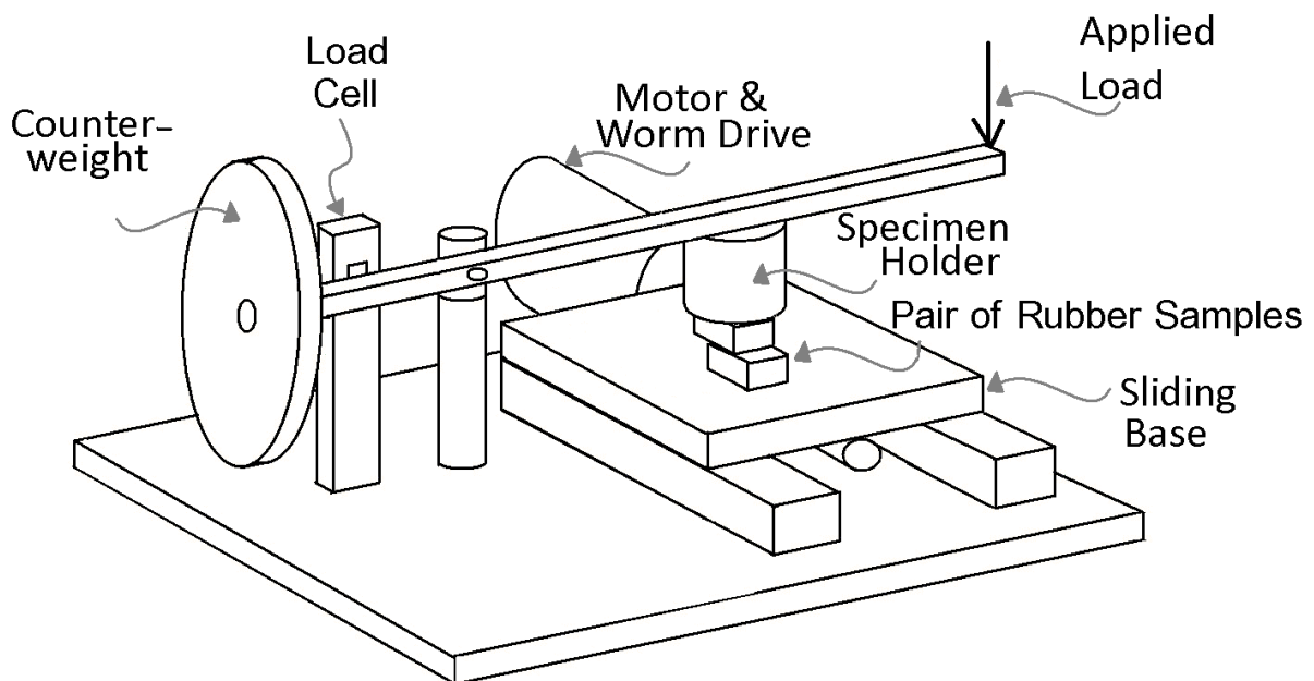
Figure 3 Experimental apparatus for husking and friction testing.
