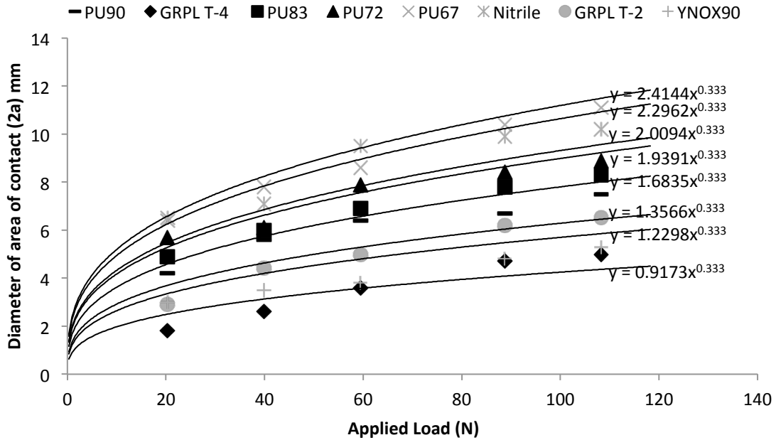
Figure 2 The diameter of the area of contact for a steel sphere pressed against the rubber samples. A power law curve fit is used to estimate the Young's modulus.
