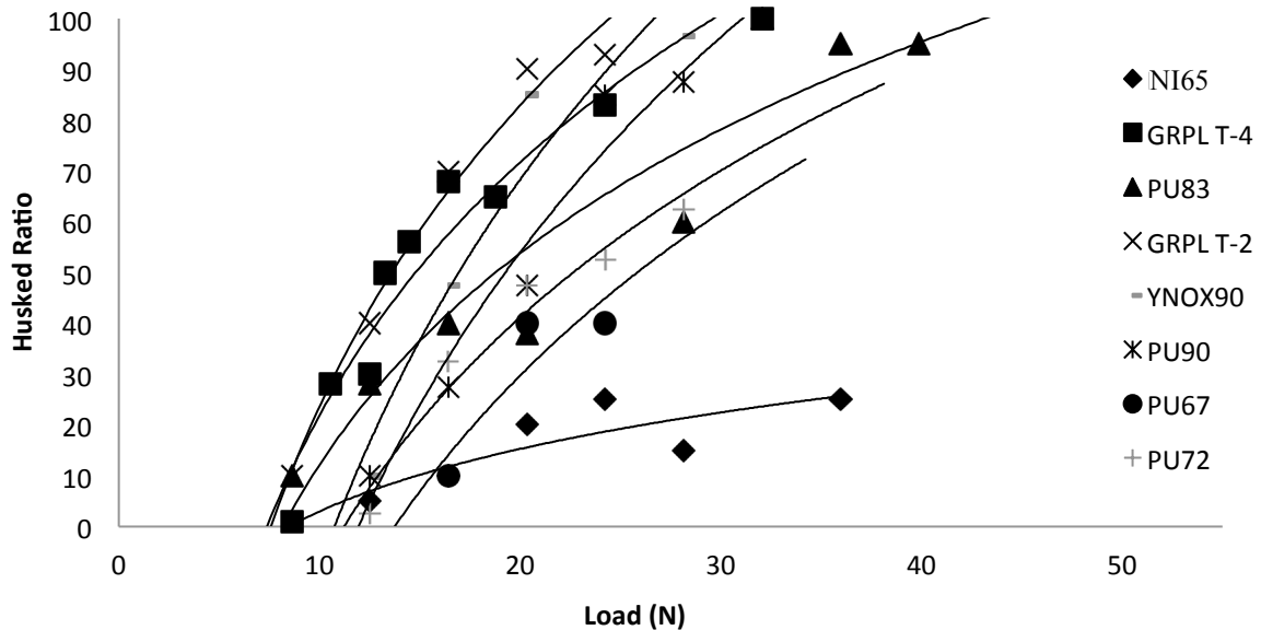
Figure 10 Graph showing husked ratio for various loads and different rubber samples
