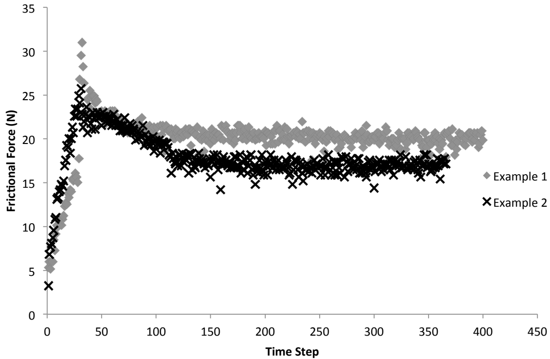
Figure 9 Frictional Force for Grain of Rice Over Test Duration
