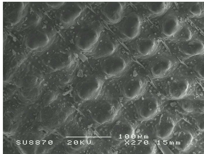
Figure 8 Electron Micrograph of Long Grain Rice Husk (Magnified)
