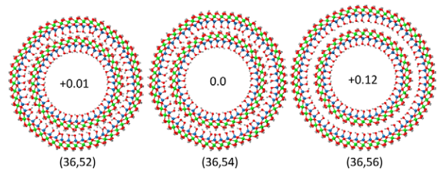
Figure 2. Front view of the optimized DW AlGe ( N_{in} , N_{out} ) NT models screened. The relative energy per (Al 2 GeO 7 H 4 ) unit (eV) is shown inside each NT-model.
