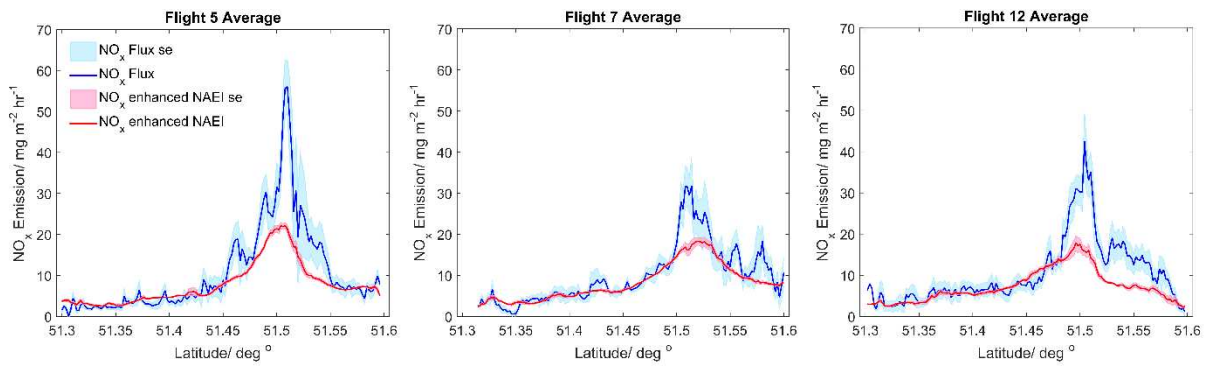
Figure 7. Average for Flight's 5, 7 and 12, measured NO x flux plotted in blue with standard error as the shaded blue area. Calculated and scaled enhanced NAEI estimates of NO x emission is plotted in red, with standard error as the shaded red area.
