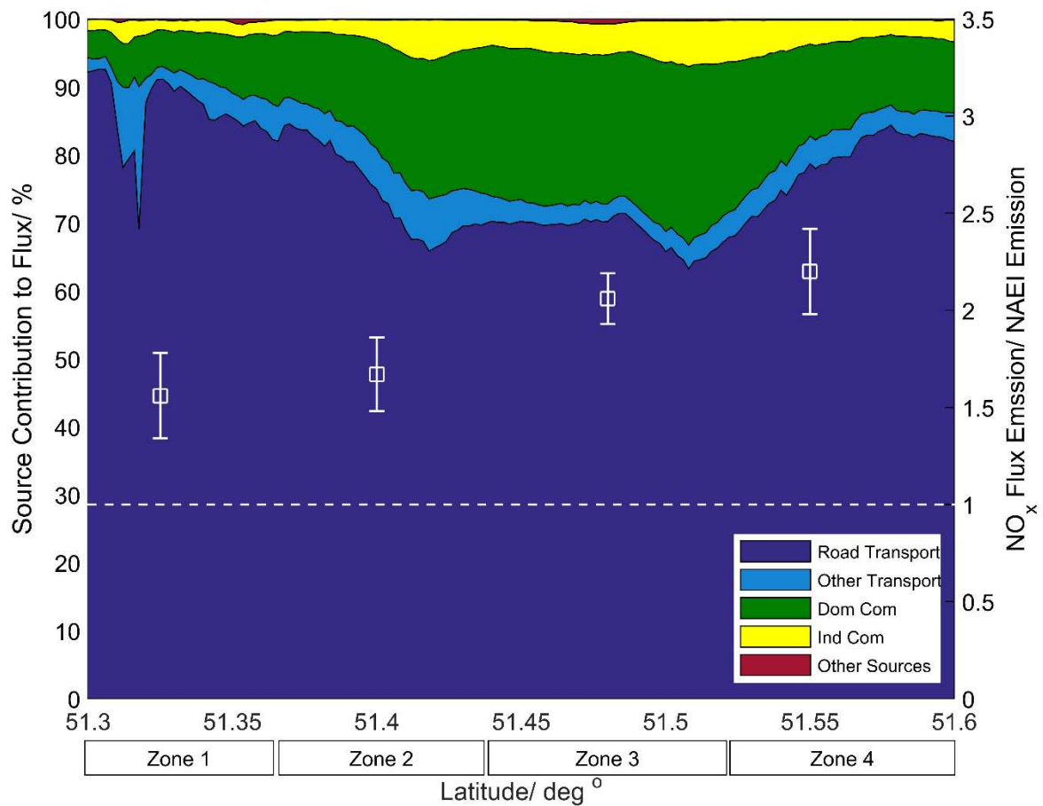
Figure 6. Calculated emission source contributions from the NAEI plotted on the first y axis, with sources being broken down into road transport; other transport (such as rail), domestic combustion, industrial combustion and other sources. Also plotted on the second y axis as white squares is the ratio of measured to NAEI estimated NO x flux, with the error bars denoting the standard error of all points included. The flight is broken into 4 zones, with 1 and 2 being SW outer London, 3 central London and 4 NE outer London.
