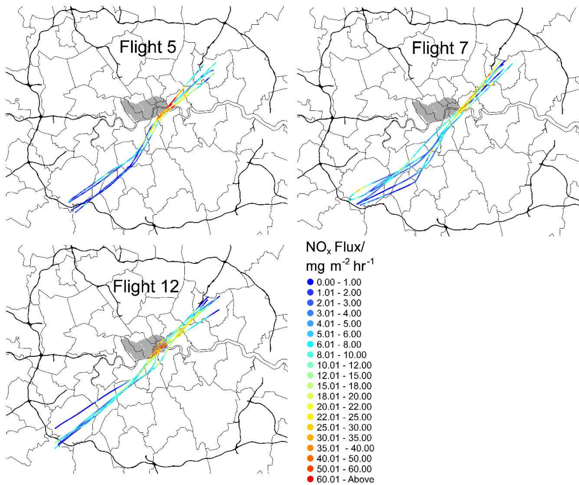
Figure 4. Tracks of all the flight legs for flights 5 (3 rd July 2013 morning), 7 (4 th July 2013 afternoon) and 12 (9 th July 2013 afternoon), mapped over Greater London, coloured to the measured NO x flux. The grey area represents London's Low Emission's Zone (LEZ).
