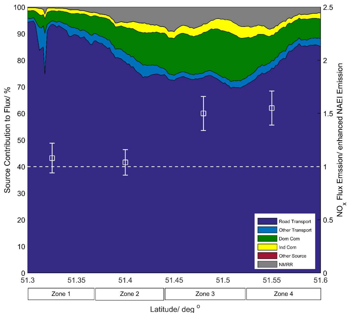
Figure 8. Calculated emission source contributions from the enhanced NAEI (see text for details) plotted on the first y axis, with sources being broken down into road transport; other transport (such as rail), domestic combustion, industrial combustion, other sources and non-road mobile machinery (NRMM). Also plotted on the second y axis as white squares is the ratio of measured to enhanced NAEI estimated NO x flux, with the error bars denoting the standard error of all points included. The flight is broken into 4 zones, with 1 and 2 being SW outer London, 3 central London and 4 NE outer London.
