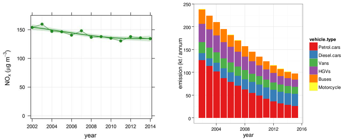
Figure 1: a) Trends in the mean concentration of NO x across 35 roadside sites in Greater London with at least 10 years of data capture, b) Projected change in urban road transport emissions split by main vehicle type from the NAEI using 2002 as a base year.
