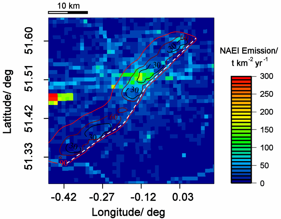
Figure 3. The contributing footprint area to a typical flight track, dependant on the prevailing wind direction and altitude of flight. The footprint is overlaid onto the NAEI at 1\ km^2 grid resolution, coloured to annual NO_x tonnage emission estimates.
