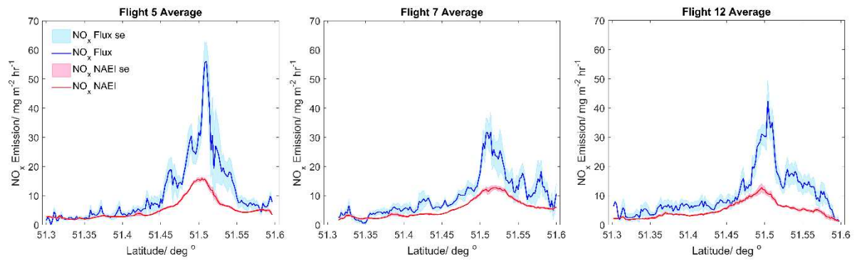
Figure 5. Average for Flight's 5, 7 and 12, measured NO x flux plotted in blue with standard error as the shaded blue area. Calculated and scaled NAEI estimates of NO x emission is plotted in red, with standard error as the shaded red area.
