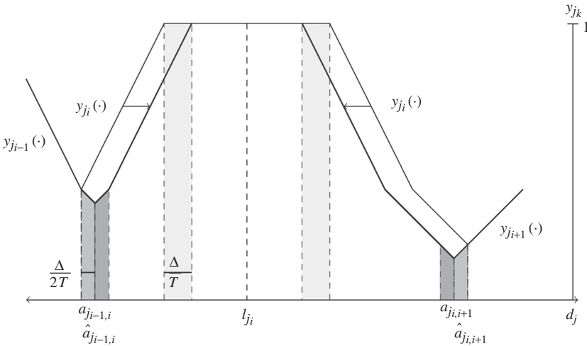
Figure 6: The effect of a marginal increase in the price charged for product j , by \Delta from p_j to \hat{p}_j . The light gray rectangles represent a loss in demand for product j . The darker gray trapezoids represent a gain in demand for product j . The lighter gray trapezoids represent a gain in demand for products j_{-1} and j_{+1} .
