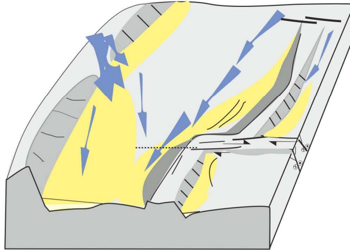
Cross-cutting faults result in lateral offset in sand-fairways although may be locally deformed with short wavelength folding and inversion structures
