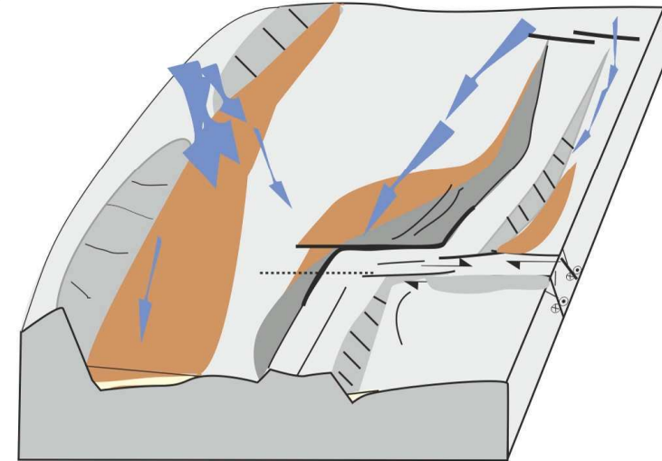
Location of sand fairways are controlled by intra-basin and basin bounding faults.
