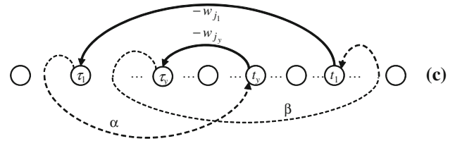
Fig. 11 Negative cycle ((t_1, \tau_1), \alpha, (t_y, \tau_y), \beta)
