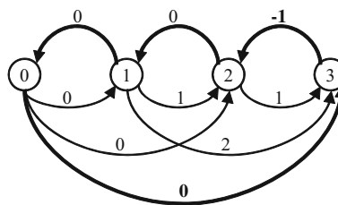
Fig. 20 A unique negative cycle for Example 9 of the left-chain type
