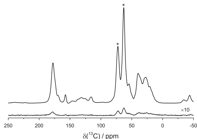
Fig. 2. ^1\text{H} - ^{13}\text{C} CP DNP spectra of bacteriorhodopsin in purple membrane using AMUPOL radical at 90 K. The unenhanced spectrum (lower) has been multiplied by 10 to allow better comparison. The two stars (*) denote glycerol peaks from the buffer. Both spectra were acquired with 256 co-added transients and a 3 s recycle delay. The enhancement achieved is approximately 120.
