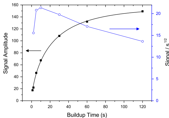
Fig. 4. ^{13}\text{C} signal build-up of furoseamide with 16 mM TEKPOL in dibromobutane, squares. The signal amplitude has been fitted to a stretched exponential with a T_{1B} of 23 s and a stretching factor \beta of 0.70. The circles show the signal per root second which is optimal for a build-up time of \sim 10 s.
