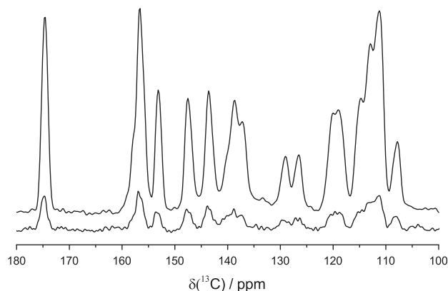
Fig. 5. ^{13}\text{C} CP MAS Spectra of furoseamide using 16 mM TEKPOL in dibromobutane as the polarising agent. 64 acquisitions with a 10 s build-up delay were acquired. The top spectrum is DNP enhanced. The enhancement achieved with this build-up time was approximately 5.5.
