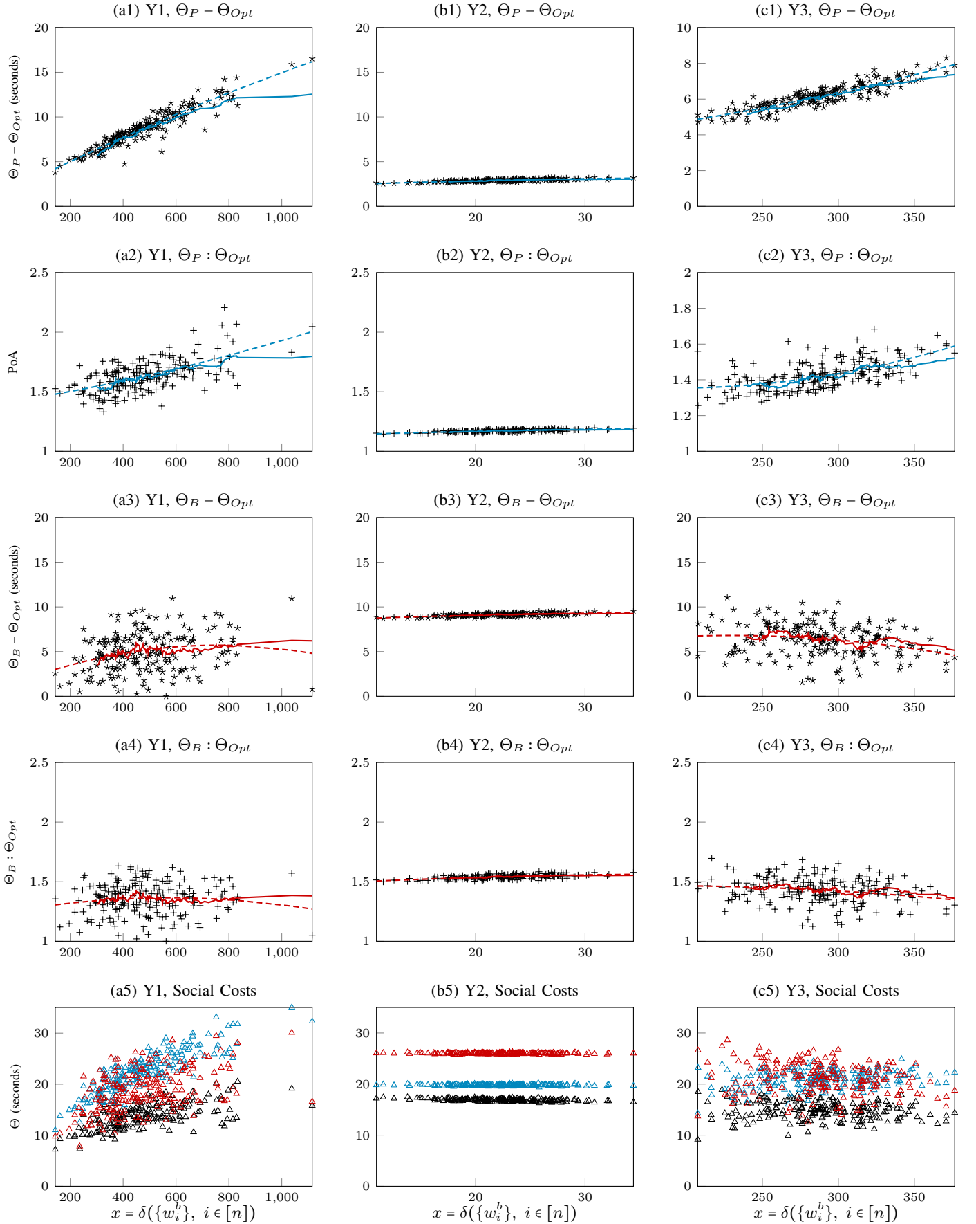
Fig. 4. Y1, Y2 and Y3. Gap between \Theta_P , \Theta_B and \Theta_{Opt} , Price of Anarchy, Social Costs.
