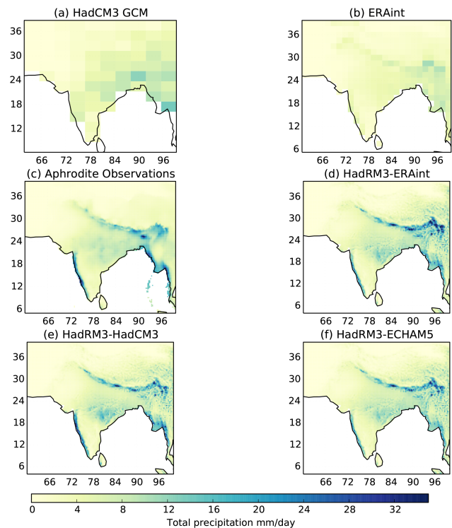
Figure 3. The spatial distribution of the seasonal mean total precipitation for the monsoon period (June, July, August, September) for the HadCM3 GCM (a), ERAint (b), APHRODITE observations (c) and the three HadRM3 simulations: HadRM3-ERAint (d), HadRM3-HadCM3 (e) and HadRM3-ECHAM5 (f).
