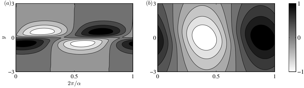
FIGURE 6. Eigenfunctions of (a) vorticity and (b) height for the most unstable modes for U(y) = \tanh y at F = 0 , M = 0 .
