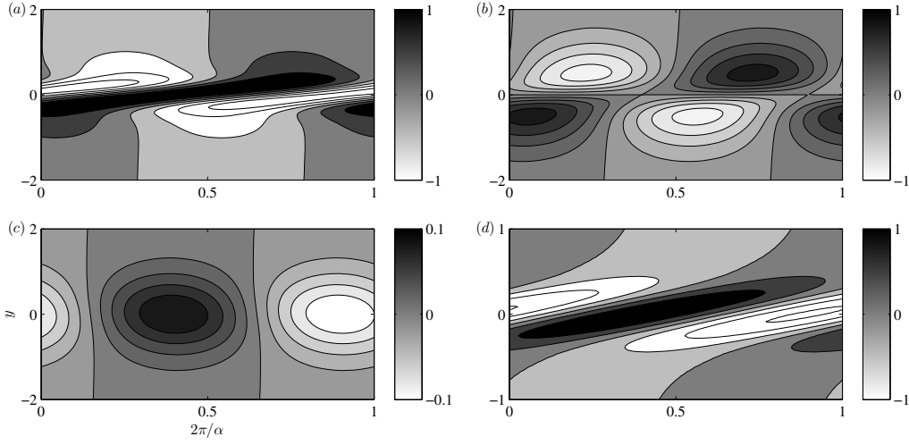
FIGURE 7. A generic vorticity budget breakdown for the case where neither F nor M is zero; shown here is F = 0.5 and M = 0.25 , with (a) \omega , (b) -\eta\Omega' , (c) F^2h\Omega , (d) M^2j/(U-c) . Notice that the vorticity contribution from the magnetic term is substantially larger than that from the shallow-water term.
