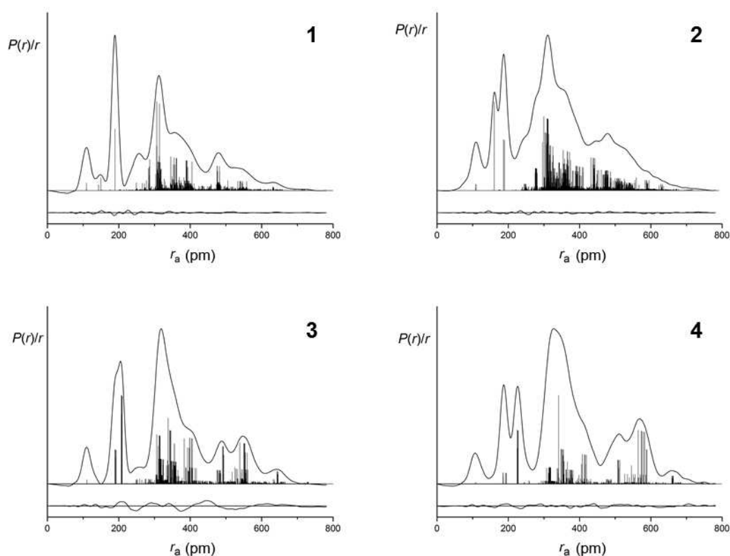
Fig. 3. Experimental and difference (experimental-minus-theoretical) radial distribution curves, P(r)/r , from the GED refinement of C(\text{Si}X\text{Me}_2)_4 [ X = \text{H} ( 1 ), \text{F} ( 2 ), \text{Cl} ( 3 ), \text{Br} ( 4 )]. Before Fourier inversion, data for 1 and 2 were multiplied by s \cdot \exp(-0.00002s^2)/(Z_C - f_C)(Z_{\text{Si}} - f_{\text{Si}}) , while data for 3 and 4 were multiplied by s \cdot \exp(-0.00002s^2)/(Z_C - f_C)(Z_X - f_X) .
