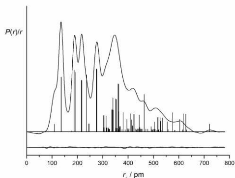
Figure 10. Experimental, theoretical and difference (experimental – theoretical) radial distribution curves for 1,2-bis(trifluoromethyl)-1,1,2,2-tetramethyldisilane.
