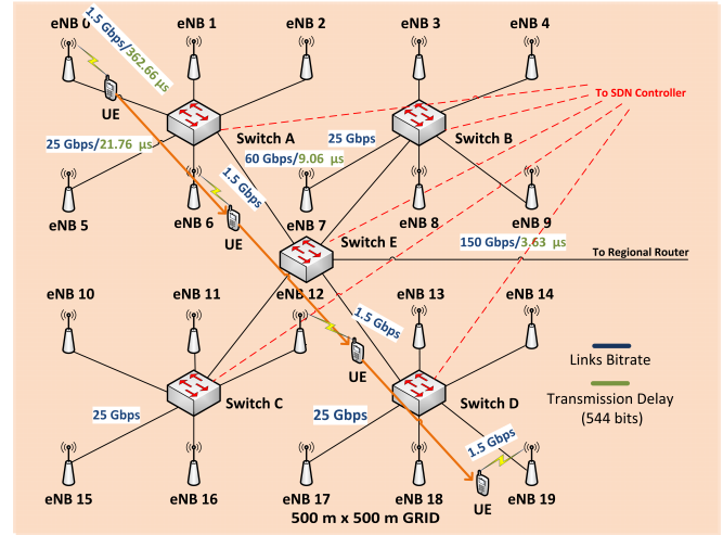
Fig. 3. Experimental topology
