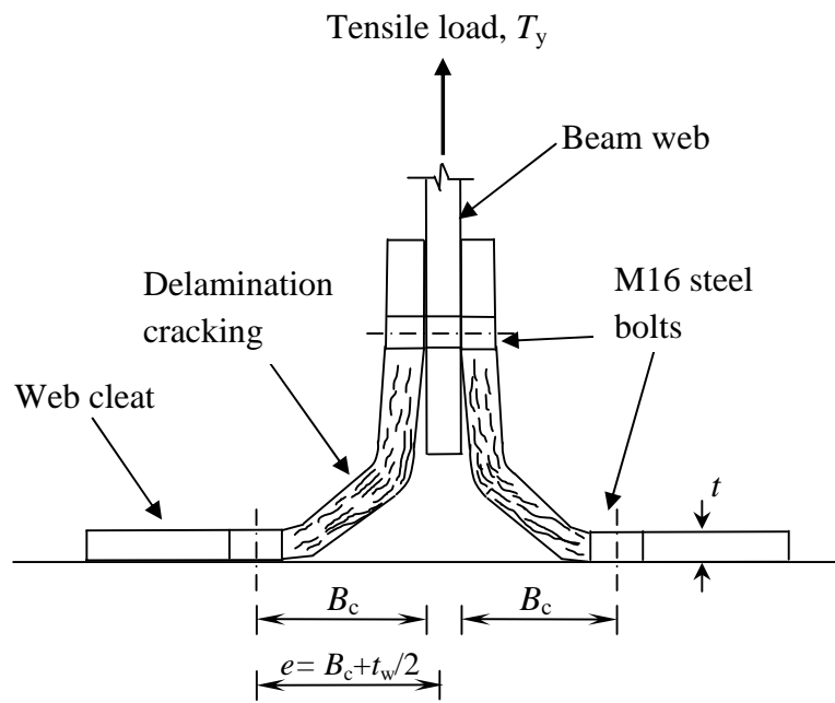
Fig. 10. Schematic line drawing of a failed web cleated joint under tensile load
