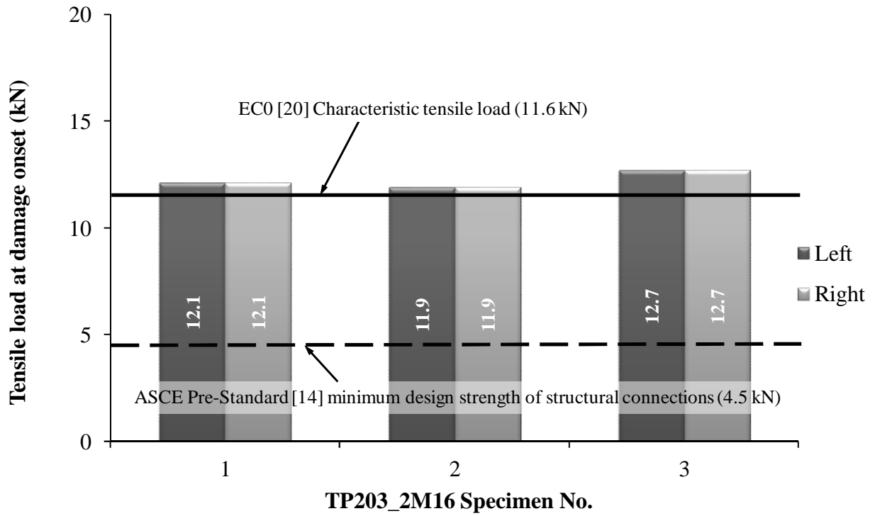
Fig. 9. Characteristic tensile loads for batch TP203_2M16.
