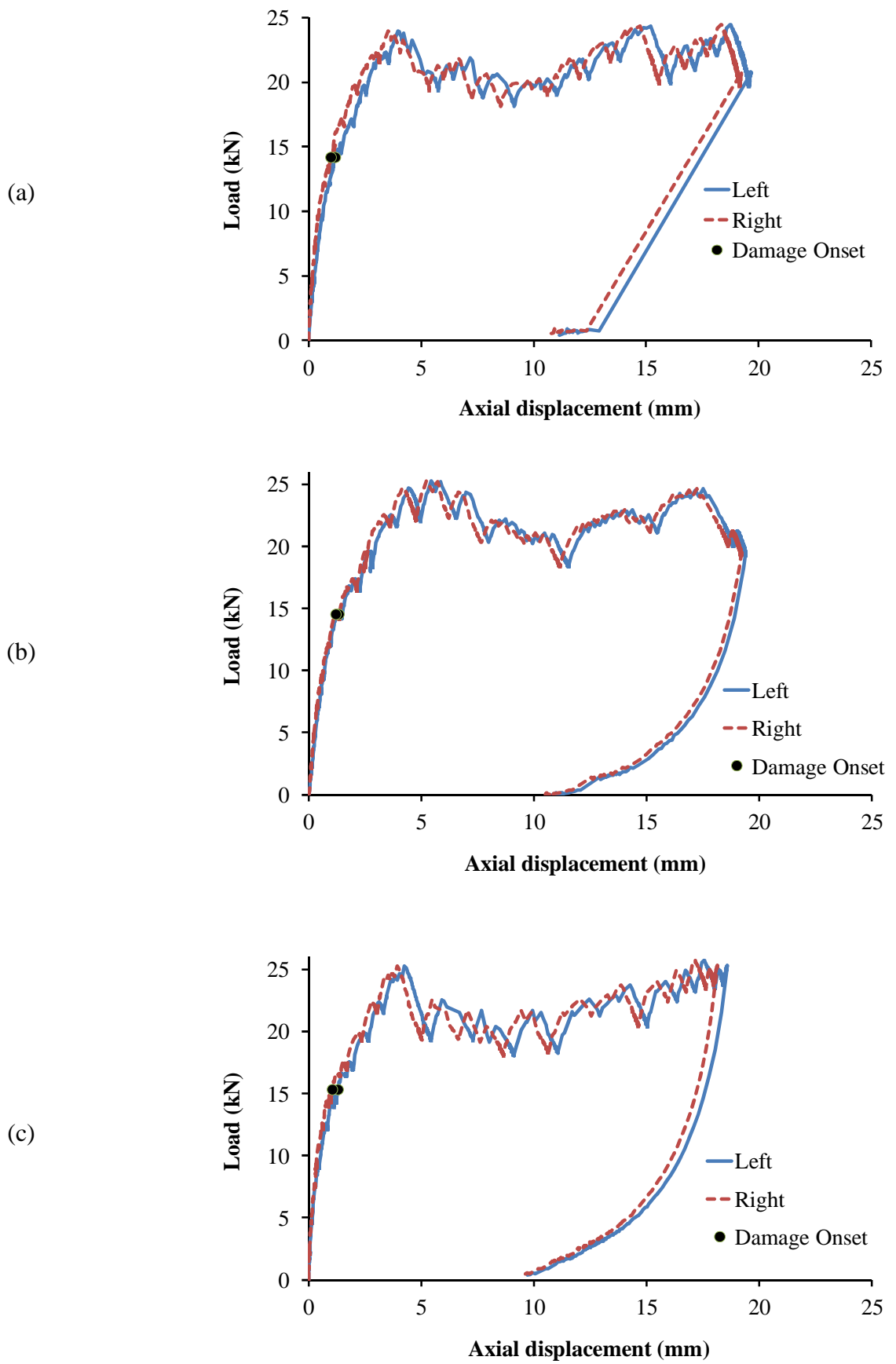
Fig. 6. Tensile load against axial displacement curves for batch TP254_3M16: (a) Specimen 1; (b) Specimen 2; (c) Specimen 3.
