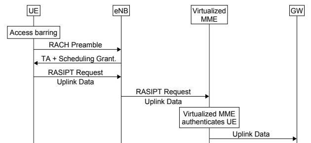
Fig. 3. RASIPT procedure sequence.
