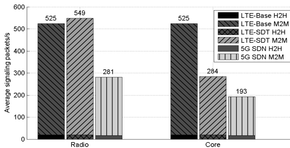
Fig. 4. Comparison of the average signaling packets/s in different parts of the network.
