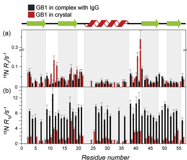
Figure 1. a) ^{15}\text{N} R_1 and b) R_{1\rho} relaxation rate measurements in 100% proton back-exchanged [ U\text{-}^2\text{H} , ^{13}\text{C} , ^{15}\text{N} ]GB1 in a complex with IgG (black) and in a GB1 crystal (red). For the severely overlapping peaks values were removed (see Figures S2–3). Experiments were performed at an 850 MHz spectrometer, 60 kHz spinning frequency, and with a 17 kHz spin-lock field for measurements in (b). The sample temperature was 27 \pm 1 °C as calculated from the chemical shift of water protons.
