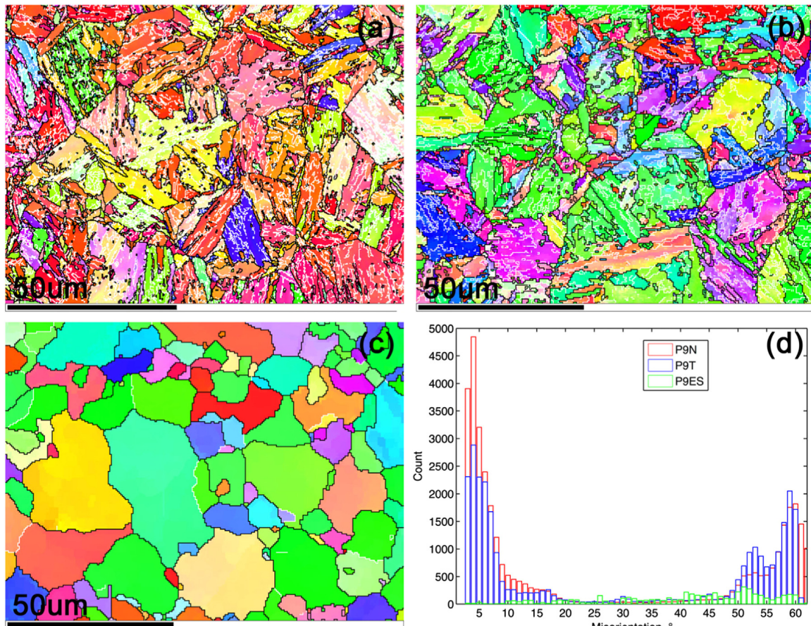
Fig. 2. Inverse pole figure map with low angle ( 3\text{--}15^\circ ) and high angle ( >15^\circ ) boundaries highlighted with white and black line respectively for P9 in different conditions: (a) as normalised, (b) as normalised and tempered and (c) ex-service P9. (d) Distribution of boundary misorientation values. Although some contrast consistent with individual laths is seen in (a) and (b) they are not clearly resolvable at these magnifications and so the features observed are lath packets or lath colonies [6].
