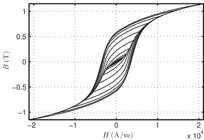
Fig. 13. A series of unbiased minor loops for different amplitude for the P9N sample.
