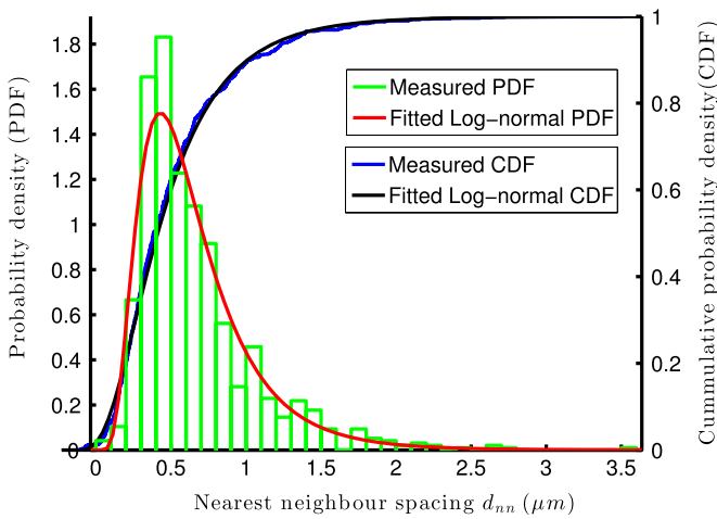
Fig. 4. Distribution of the nearest-neighbour inter-particle spacing for the precipitates within the grains of the service-exposed P9 (P9ES).
