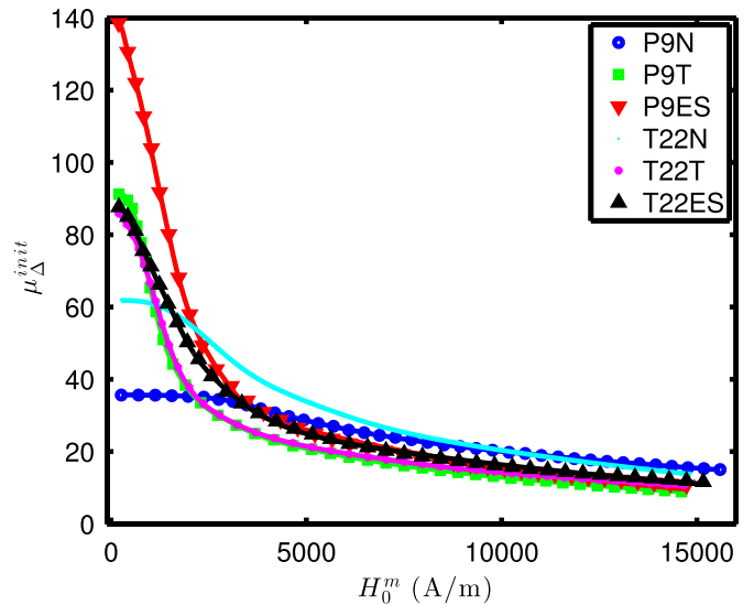
Fig. 17. Incremental permeability for the biased minor loop excursions from the initial magnetisation curve as a function of the DC bias field H_0^m and fitting with a multi-term Gaussian function (solid lines).
