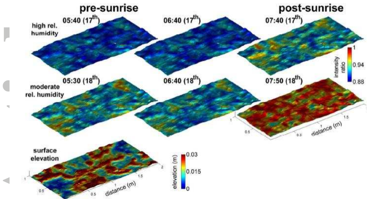
Figure 14 Ridged crust topography coloured by the early morning change in surface moisture (R4 and R5). Upper row (R4) shows increased relative wetting of ridged areas under high relative humidity (maximum 83%) and the surface takes longer to dry after dawn. Similar spatial response under moderate relative humidity (R5; middle row; maximum 70%), but faster drying after dawn. Sunrise was at 6:09 and 6:08 for the 17 th and 18 th respectively. Corresponding climate conditions are shown in Figure 13.
