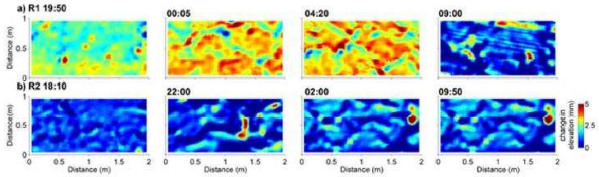
Figure 12 Nocturnal change in surface elevation from early evening (left) to after dawn (right) for R1 and R2. Sunset and sunrise times are indicated in Table 1. Plots correspond to the same areas shown in Figures 10 and 11, and are coloured by change between scanned topography overnight and the previous day. Red indicates surface expansion greater than 5 mm. Refer to Figure 9 for corresponding temperature and relative humidity.
