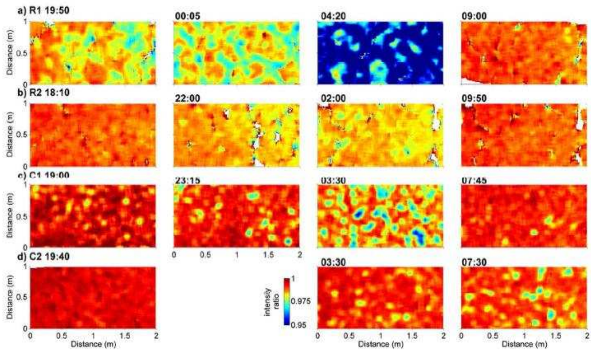
Figure 11 Nocturnal trends in surface moisture for each nocturnal crust section, coloured by the TLS ratio of the intensity of the surface during the night and day. Sunset and sunrise times are indicated in Table 1. Blue indicates a higher relative increase in moisture, red little change in moisture overnight. The time each scan was collected is shown above each plot. Corresponding climatic conditions and surface elevations are indicated in Figures 9 and 10 respectively.
