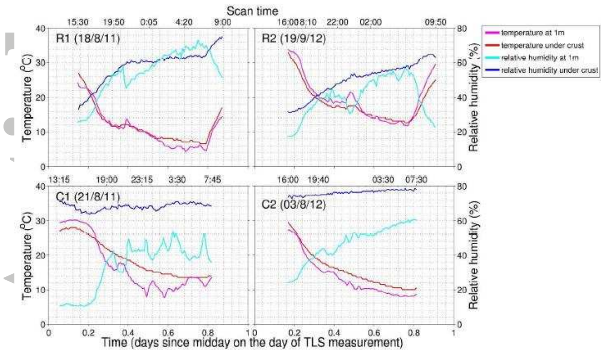
Figure 9 Overnight temperature and relative humidity above and below the crust for ridged (R1, R2) and continuous (C1, C2) surfaces during TLS scanning. Scan time relates to the times when repeat surface scans were undertaken to extract moisture and elevation data corresponding to the DEMs. Exact sunset and sunrise times are indicated in Table 1 (approximately 18:00 and 06:00).
