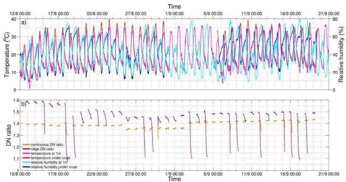
Figure 7 a) Temperature and relative humidity above and below the crust at M1 during August and September 2012. b) Nocturnal digital number (DN) ratios of ridged and continuous crust and calibration tile from infra-red (IR) flash camera.
