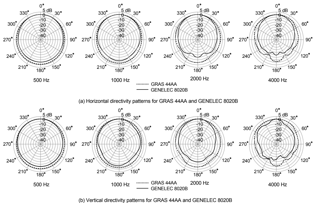
Fig. 3. The horizontal and vertical directivity patterns of the artificial mouth GRAS 44AA and monitor loudspeaker 8020B.
