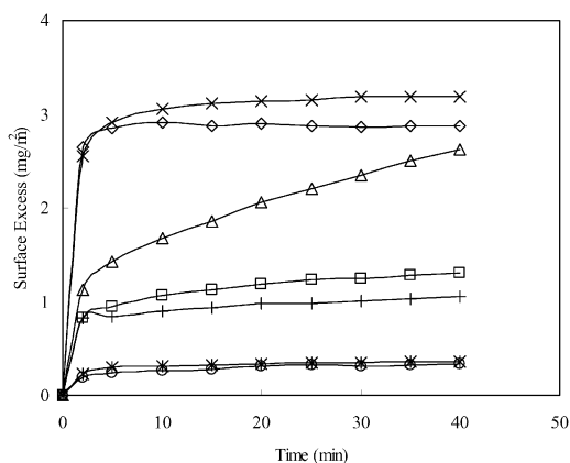
Fig. 5 The adsorption isotherm of V_6K at 100 \mu\text{g ml}^{-1} (x) and C_{12}TAB at 0.128 mM (o); 2.63 mM (*); 12 mM (□). The co-adsorption was at the molar ratio of C_{12}TAB and V_6K of 1:1 (◇), 20:1 (Δ) and 94:1 (+). V_6K was fixed at 100 \mu\text{g ml}^{-1} (0.128 mM), all at pH 7.
