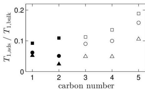
Fig. 6 The ratio of surface to bulk relaxation times T_{1,ads}/T_{1,bulk} for the individual carbon atoms in 1-pentene adsorbed on \theta -Al 2 O 3 with a surface coverage of approximately 1 ML (squares), 0.5 ML (circles), and 0.2 ML (triangles). Solid symbols represent olefinic carbons and open symbols represent aliphatic carbons.
