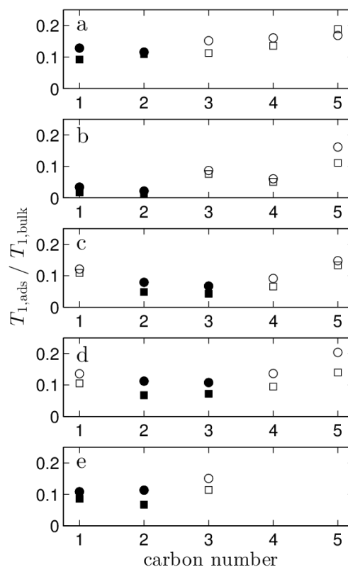
Fig. 2 The ratio of surface to bulk relaxation times T_{1,ads}/T_{1,bulk} for the individual carbon atoms in (a) 1-pentene, (b) 1-pentyne, (c) cis -2-pentene, (d) trans -2-pentene, and (e) 1,4-pentadiene adsorbed on \theta -Al 2 O 3 (squares) and \gamma -Al 2 O 3 (circles). The carbon numbers correspond to the schematic diagrams in Fig. 1. Solid symbols represent olefinic or acetylinic carbons associated with the unsaturated carbon-carbon bonds, and open symbols represent aliphatic carbons.
