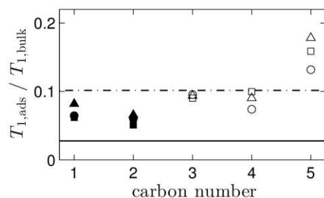
Fig. 11 The ratio of surface to bulk relaxation times T_{1,ads}/T_{1,bulk} for the individual carbon atoms in 1-pentene co-adsorbed with benzene and cyclohexane on \theta -Al 2 O 3 . Data are shown for adsorption of 0.5 ML 1-pentene following adsorption of 0.9 ML cyclohexane (circles), and adsorption of 0.5 ML 1-pentene following adsorption of 0.9 ML benzene (triangles). For comparison, data for the adsorption of 0.5 ML 1-pentene only (squares) are repeated from Fig. 6. Solid symbols represent olefinic carbons and open symbols represent aliphatic carbons. The single T_{1,ads}/T_{1,bulk} ratios for benzene (solid line) and cyclohexane (dash-dot line) are included.
