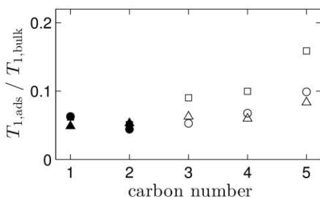
Fig. 7 The ratio of surface to bulk relaxation times T_{1,ads}/T_{1,bulk} for the individual carbon atoms in 1-pentene adsorbed on \theta -Al 2 O 3 with a surface coverage of 0.5 ML at 20°C (squares), 10°C (circles), and 0°C (triangles). Solid symbols represent olefinic carbons and open symbols represent aliphatic carbons.
