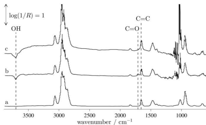
Fig. 3 DRIFTS of 1-pentene adsorbed over (a) KBr, (b) \theta -Al 2 O 3 , and (c) \gamma -Al 2 O 3 at 35°C. There is no significant change in band position with surface and the \nu (C=C) band is observed at 1647 cm -1 in all cases. The \nu (C=O) band observed at 1705 cm -1 over \theta -Al 2 O 3 may be attributable to impurities or partial oxidation of the 1-pentene. The \nu (OH) band is observed on both alumina surfaces even after treatment to remove hydroxyl groups. Spectra are displayed as \log(1/R) , where R is the ratio of the relative reflectance of a surface with 1-pentene adsorbed to the relative reflectance of a clean surface.
