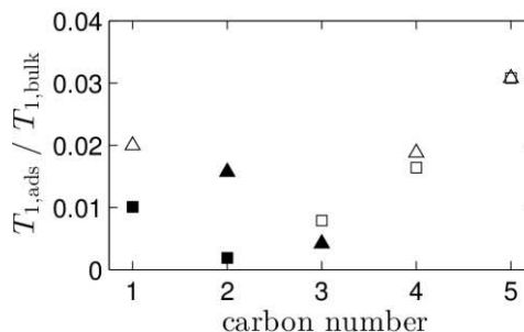
Fig. 8 The ratio of surface to bulk relaxation times T_{1,ads}/T_{1,bulk} for the individual carbon atoms observed on pre-heated \theta -Al 2 O 3 at 400°C after the adsorption of 0.5 ML 1-pentene. 1-pentene (squares) and trans -2-pentene (triangles) were
