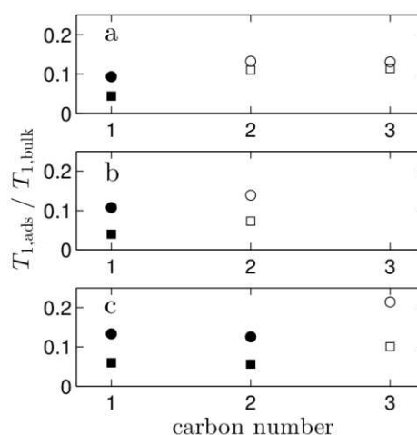
Fig. 4 The ratio of surface to bulk relaxation times T_{1,ads}/T_{1,bulk} for the individual carbon atoms in (a) cyclohexene, (b) 1,4-cyclohexadiene, and (c) 1,3-cyclohexadiene adsorbed on \theta -Al 2 O 3 (squares) and \gamma -Al 2 O 3 (circles). The carbon numbers correspond to the schematic diagrams in Fig. 1. Solid symbols represent olefinic carbons associated with the unsaturated carbon-carbon double bonds, and open symbols represent aliphatic carbons.
