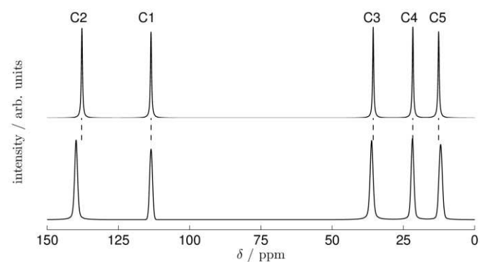
Fig. 5 ^{13}C spectra for 1-pentene (top) as bulk liquid and (bottom) adsorbed on \theta - Al_2O_3 . The dashed lines correspond to the position of the resonance lines in the bulk liquid to indicate the change in chemical shift that occurs on adsorption.
