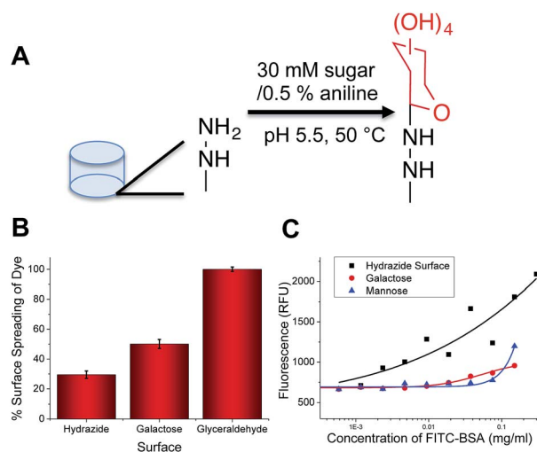
Fig. 1 Fabrication of glycosylated 96-well plates. (A) Hydrazide-carbohydrate coupling; (B) dye spreading assay showing relative hydrophilicity of surfaces; (C) non-specific binding of fluorescently-labelled bovine serum albumin onto different surfaces following 30 minutes incubation and washing.
