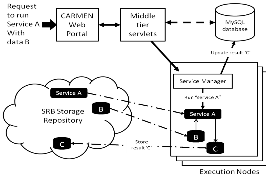
Figure 7 - CARMEN Service Dynamic Deployment
