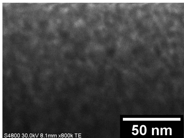
Fig. 8 A TEM image of the inner section of a single SnO 2 /SiO 2 composite fiber calcined at 500 °C.
