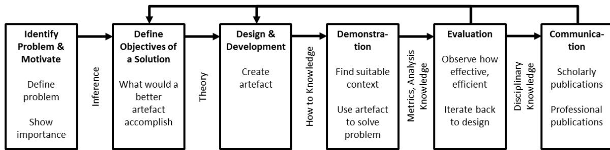
Figure 1. The design science research process, adapted from Peffers et al. (2007, fig. 1).
