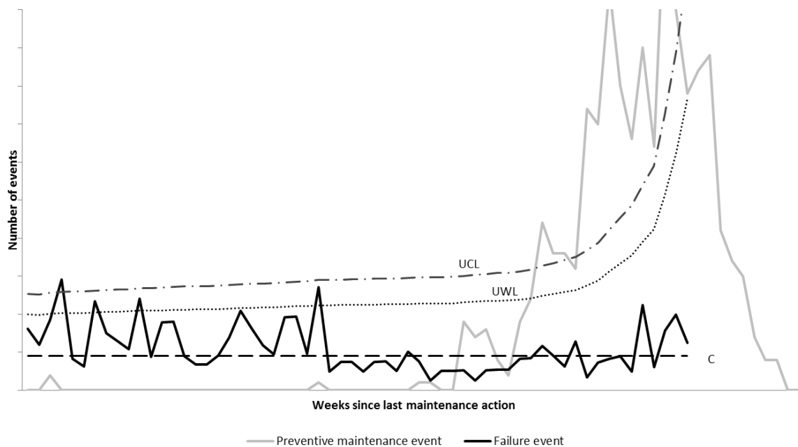
Figure 6. The measured outcomes for a main component, showing signs of maintenance induced failures.
