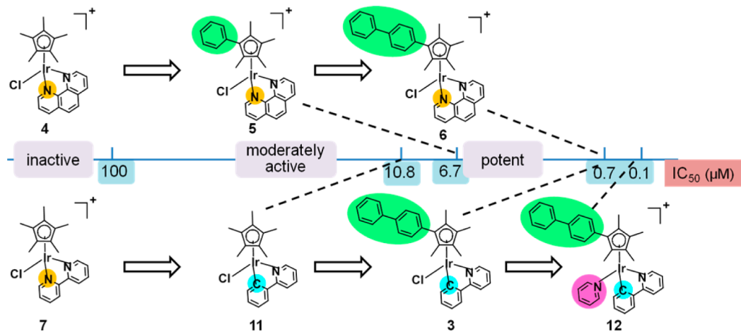
Figure 8. Comparison of cytotoxicity of [(\eta^5\text{-Cp}^*)\text{Ir}(\text{L}^{\text{A}}\text{L}')\text{Z}]^{0/+} complexes against A2780 cancer cells. Inactive: <50% growth inhibition at 100 \mu\text{M} . Moderate: 80% to 50% growth inhibition at 50 \mu\text{M} . Potent: >50% growth inhibition at 5 \mu\text{M} .
