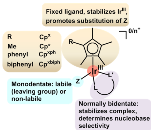
Figure 3. General structure of half-sandwich \text{Ir}^{\text{III}} cyclopentadienyl complexes. The ligands tune the chemical and biological activity.
