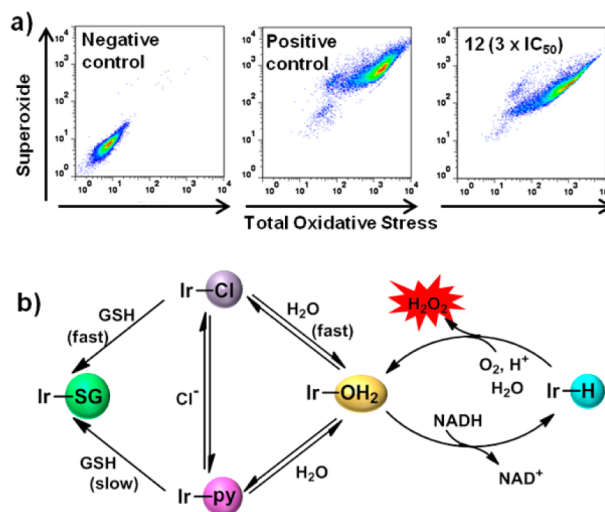
Figure 16. (a) ROS levels in A2780 cells induced by 12 after 1 h exposure at 310 K. Adapted from ref 34. (b) Reactions of Ir III pyridine complex 12 and its Cl analogue and possible pathways for generation of H 2 O 2 . More details of hydride transfer from NADH to Ir are in Figure 19.
