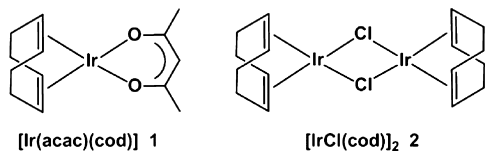
Figure 2. Early \text{Ir}^{\text{I}} anticancer compounds.
