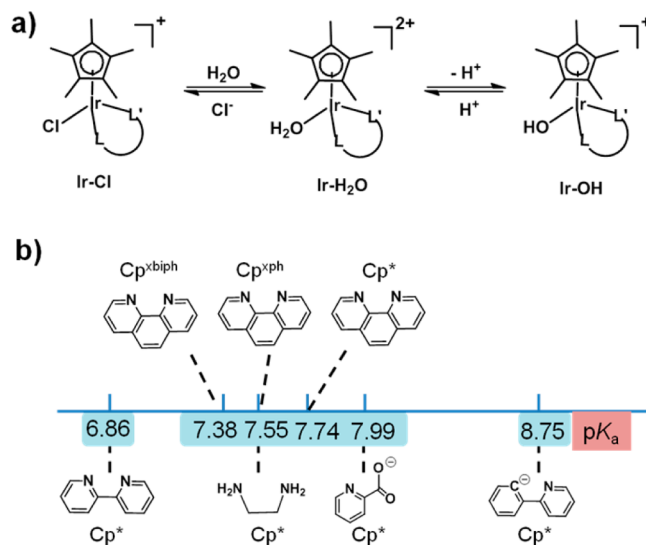
Figure 6. (a) \text{Cp}^* Ir aqua species. (b) Effects of ligands on \text{pK}_a values of aqua complexes \text{Ir}-\text{H}_2\text{O} .
