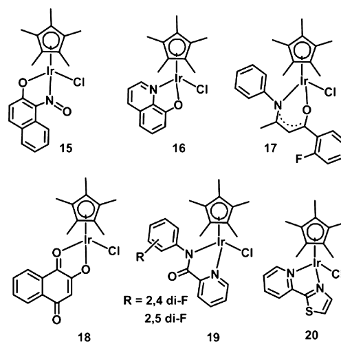
Figure 15. Cp* Ir III anticancer complexes containing N ^ O-, O ^ O-, or N ^ N-chelating ligands.
