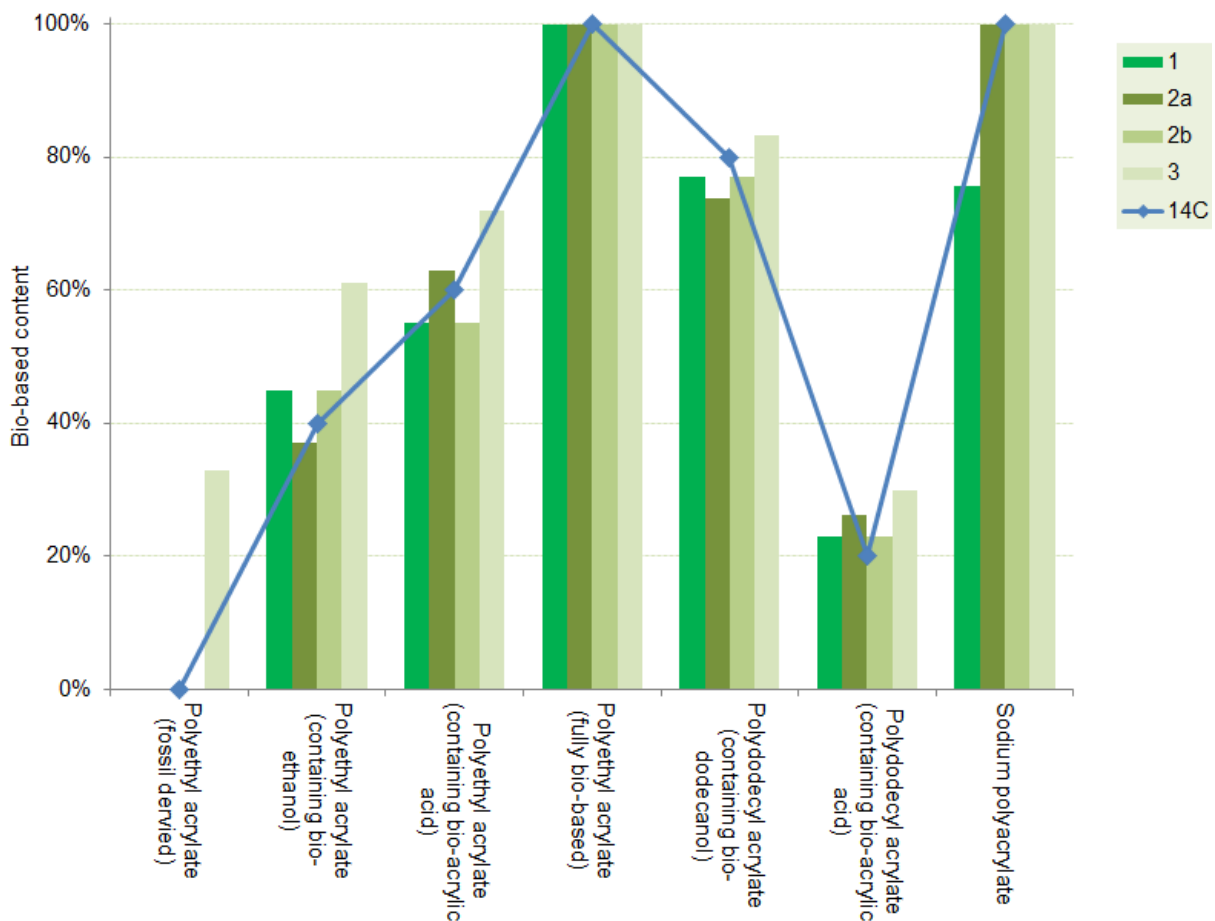
Figure 4-18 A summary of bio-based content atom connectivity method results for polyacrylates.
