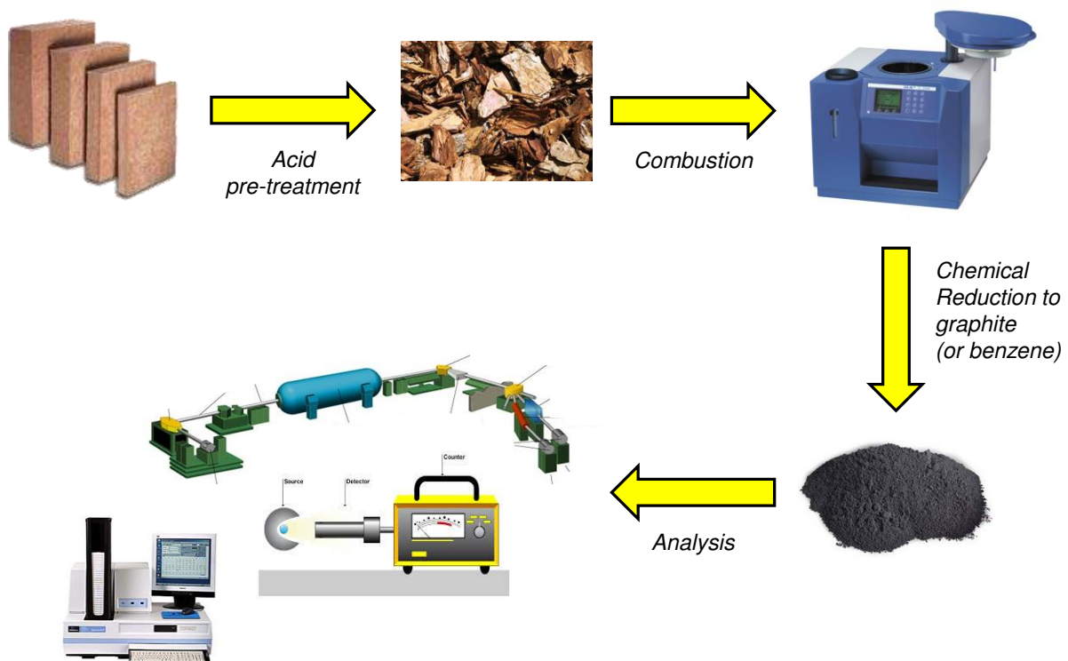
Figure 2-1 A schematic of the radiocarbon method principle of bio-based carbon content determination.
