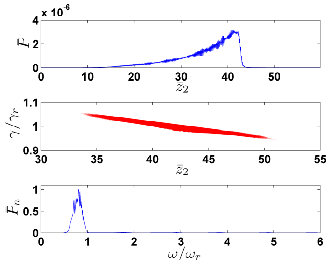
Figure 2: As Fig. 1 but for 3D Puffin simulation with the parameters of Table 1.
