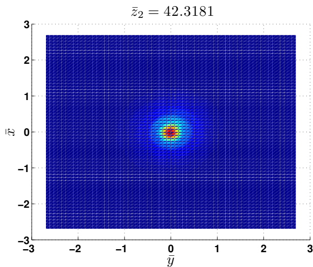
Figure 3: Transverse scaled intensity at \bar{z}_2 \approx 43.5 from 3D Puffin simulation with the parameters of Table 1.
