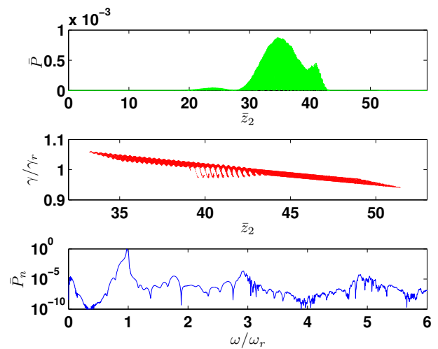
Figure 1: Scaled Power (top), electron phase space (middle) and scaled spectral power (bottom) from a 1D simulation of the parameters in Table 1. (Note the different scale in \bar{z}_2 for the plot of electron phase-space).
